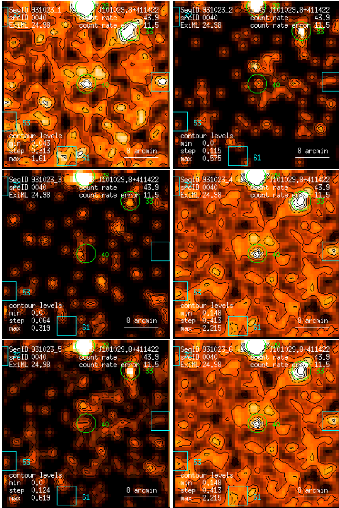
Figure 40: RASS 931023: detection 0040: band rate images, Gaussian filter: (1) PSPC channels 11 – 41, (2) 52 – 90, (3) 91 – 201, (4) 11 – 235, (5) 52 – 201, (6) 11 – 201. Broad band rates in counts/ks. Band rate contour levels in counts/ks/arcmin 2 .
