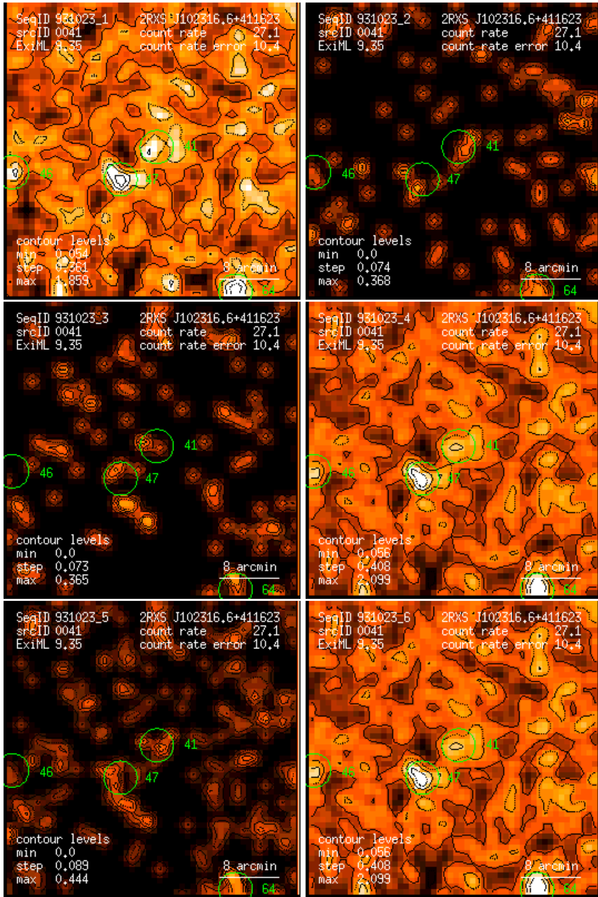
Figure 41: RASS 931023: detection 0041: band rate images, Gaussian filter: (1) PSPC channels 11 – 41, (2) 52 – 90, (3) 91 – 201, (4) 11 – 235, (5) 52 – 201, (6) 11 – 201. Broad band rates in counts/ks. Band rate contour levels in counts/ks/arcmin 2 .
