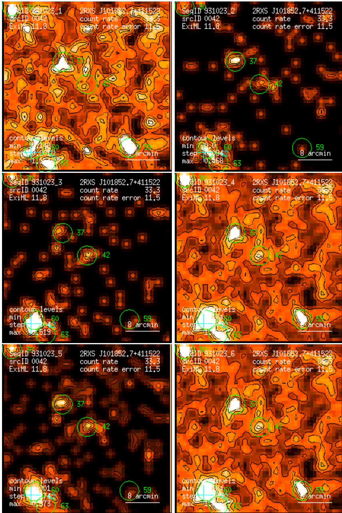
Figure 42: RASS 931023: detection 0042: band rate images, Gaussian filter: (1) PSPC channels 11 – 41, (2) 52 – 90, (3) 91 – 201, (4) 11 – 235, (5) 52 – 201, (6) 11 – 201. Broad band rates in counts/ks. Band rate contour levels in counts/ks/arcmin 2 .
