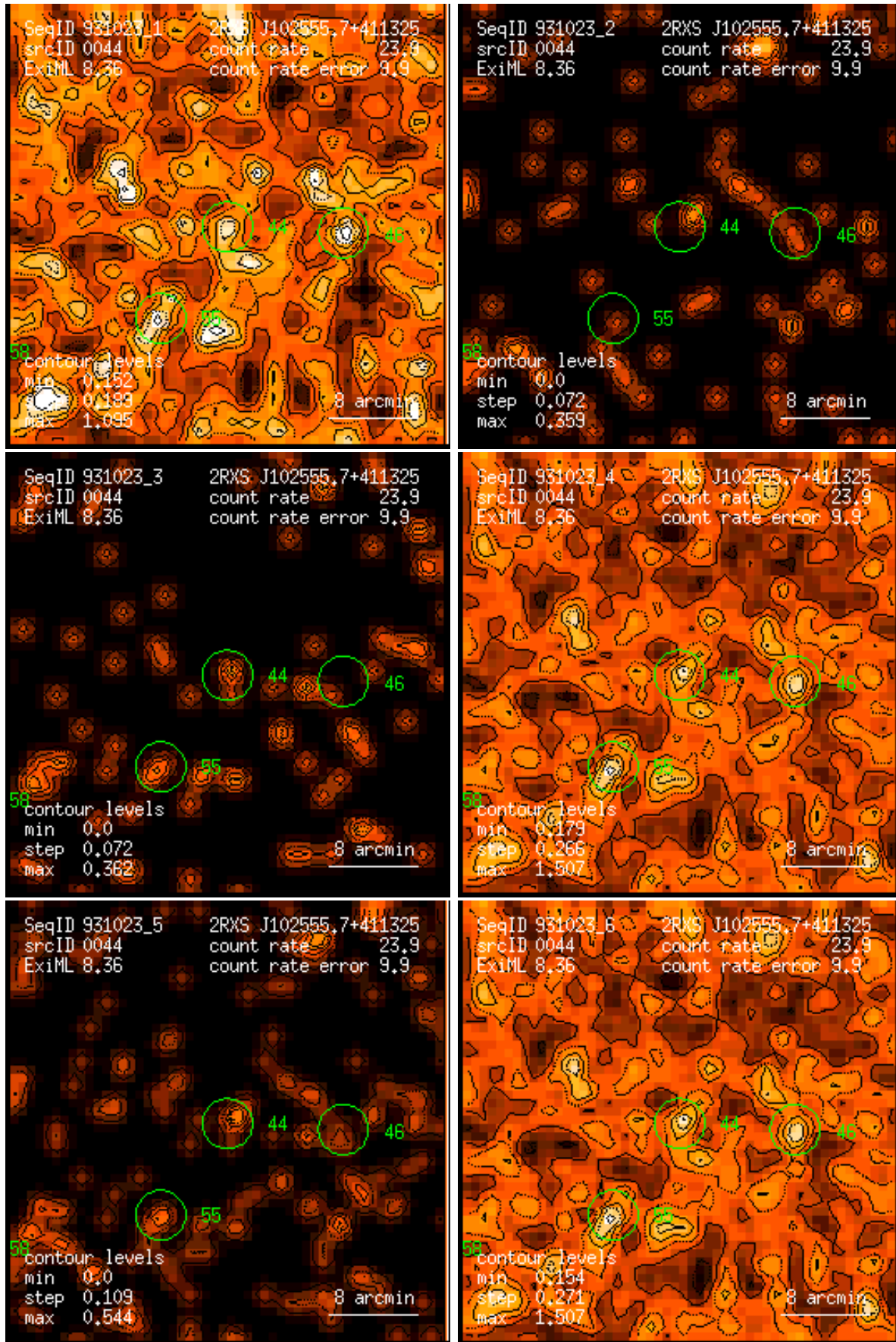
Figure 44: RASS 931023: detection 0044: band rate images, Gaussian filter: (1) PSPC channels 11 – 41, (2) 52 – 90, (3) 91 – 201, (4) 11 – 235, (5) 52 – 201, (6) 11 – 201. Broad band rates in counts/ks. Band rate contour levels in counts/ks/arcmin 2 .
