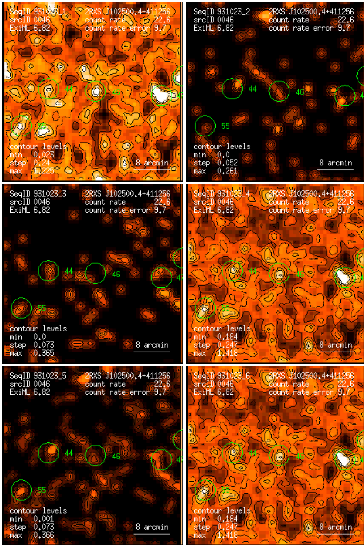
Figure 46: RASS 931023: detection 0046: band rate images, Gaussian filter: (1) PSPC channels 11 – 41, (2) 52 – 90, (3) 91 – 201, (4) 11 – 235, (5) 52 – 201, (6) 11 – 201. Broad band rates in counts/ks. Band rate contour levels in counts/ks/arcmin 2 .
