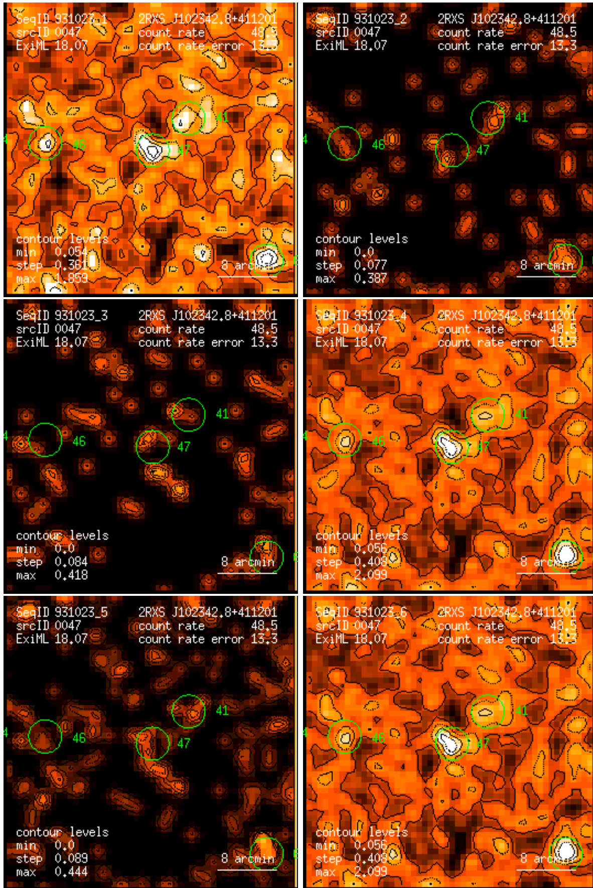
Figure 47: RASS 931023: detection 0047: band rate images, Gaussian filter: (1) PSPC channels 11 – 41, (2) 52 – 90, (3) 91 – 201, (4) 11 – 235, (5) 52 – 201, (6) 11 – 201. Broad band rates in counts/ks. Band rate contour levels in counts/ks/arcmin 2 .
