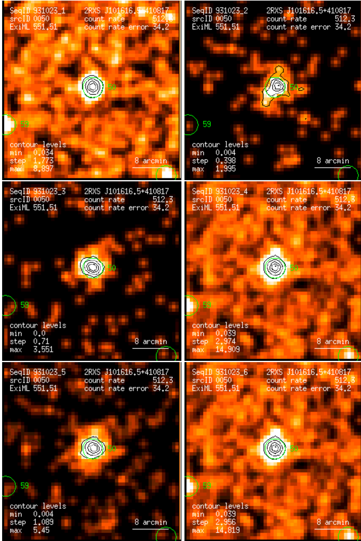
Figure 50: RASS 931023: detection 0050: band rate images, Gaussian filter: (1) PSPC channels 11 – 41, (2) 52 – 90, (3) 91 – 201, (4) 11 – 235, (5) 52 – 201, (6) 11 – 201. Broad band rates in counts/ks. Band rate contour levels in counts/ks/arcmin 2 .
