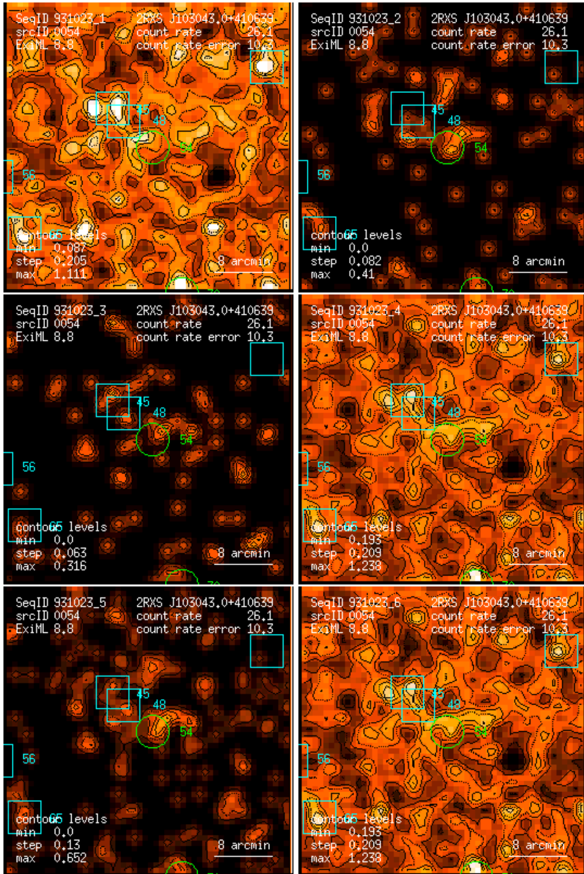
Figure 54: RASS 931023: detection 0054: band rate images, Gaussian filter: (1) PSPC channels 11 – 41, (2) 52 – 90, (3) 91 – 201, (4) 11 – 235, (5) 52 – 201, (6) 11 – 201. Broad band rates in counts/ks. Band rate contour levels in counts/ks/arcmin 2 .
