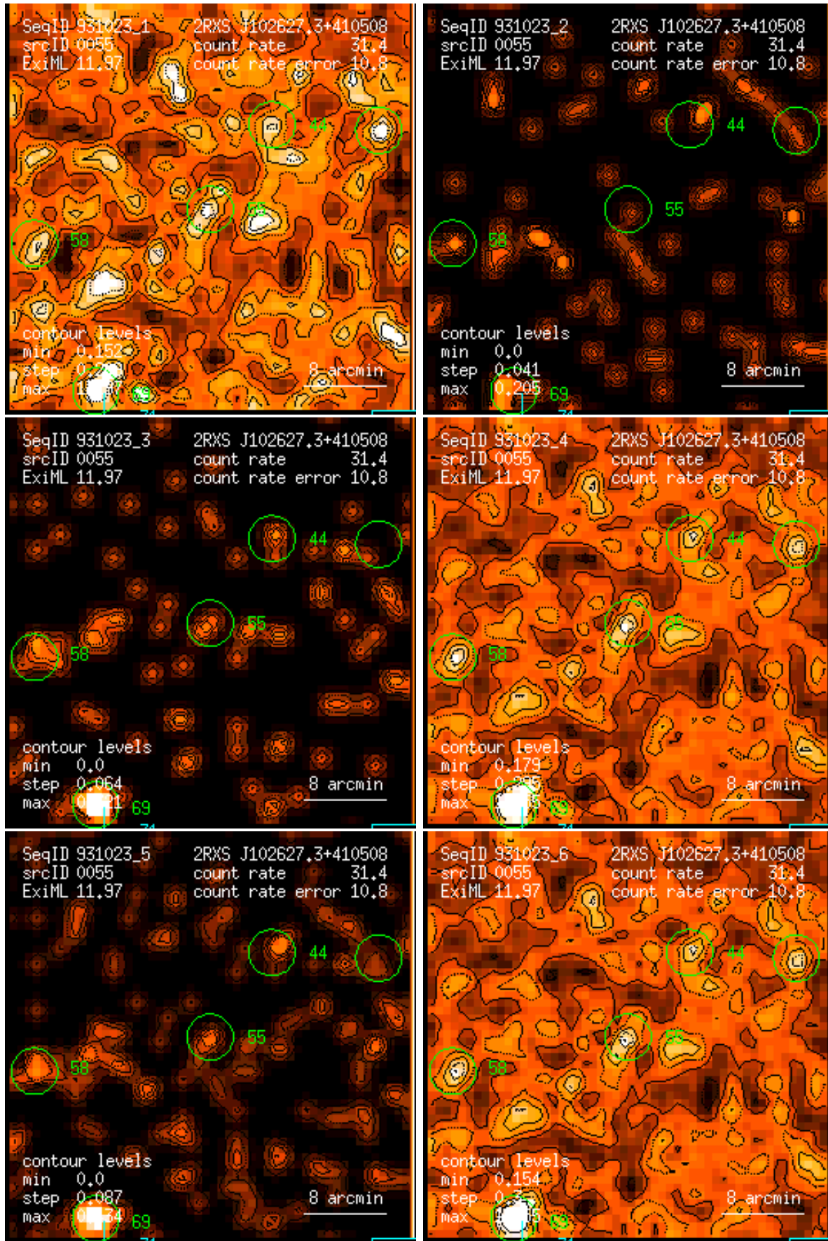
Figure 55: RASS 931023: detection 0055: band rate images, Gaussian filter: (1) PSPC channels 11 – 41, (2) 52 – 90, (3) 91 – 201, (4) 11 – 235, (5) 52 – 201, (6) 11 – 201. Broad band rates in counts/ks. Band rate contour levels in counts/ks/arcmin 2 .
