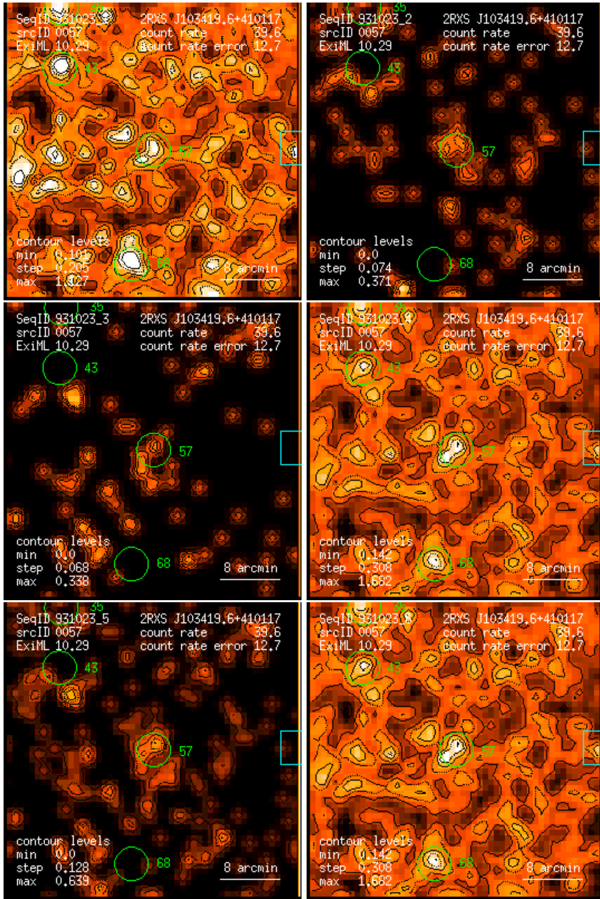
Figure 57: RASS 931023: detection 0057: band rate images, Gaussian filter: (1) PSPC channels 11 – 41, (2) 52 – 90, (3) 91 – 201, (4) 11 – 235, (5) 52 – 201, (6) 11 – 201. Broad band rates in counts/ks. Band rate contour levels in counts/ks/arcmin 2 .
