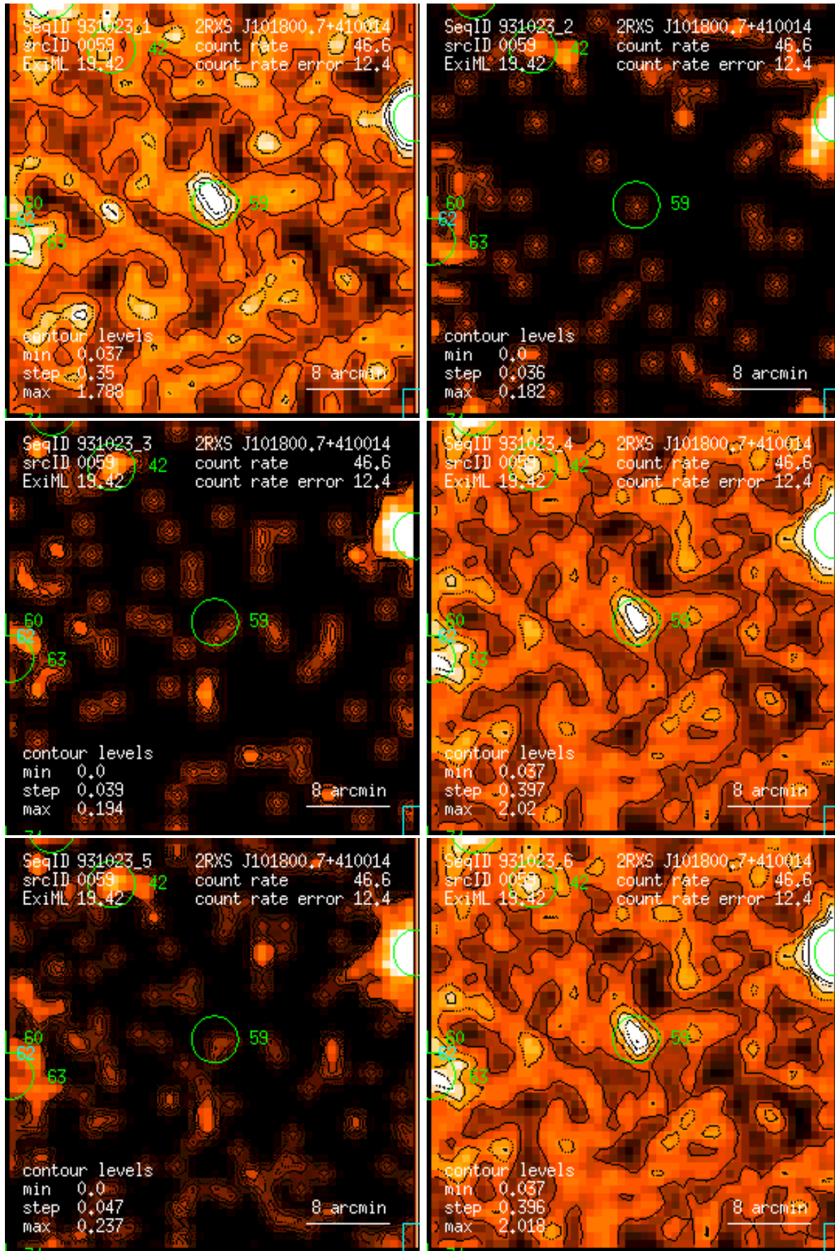
Figure 59: RASS 931023: detection 0059: band rate images, Gaussian filter: (1) PSPC channels 11 – 41, (2) 52 – 90, (3) 91 – 201, (4) 11 – 235, (5) 52 – 201, (6) 11 – 201. Broad band rates in counts/ks. Band rate contour levels in counts/ks/arcmin 2 .
