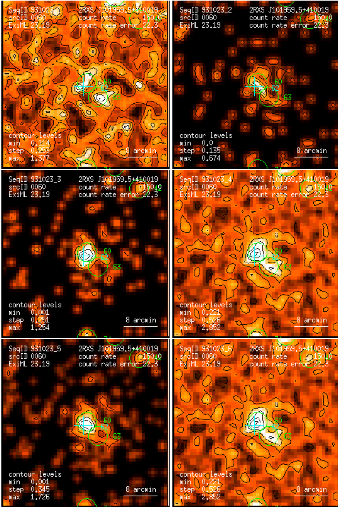
Figure 60: RASS 931023: detection 0060: band rate images, Gaussian filter: (1) PSPC channels 11 – 41, (2) 52 – 90, (3) 91 – 201, (4) 11 – 235, (5) 52 – 201, (6) 11 – 201. Broad band rates in counts/ks. Band rate contour levels in counts/ks/arcmin 2 .
