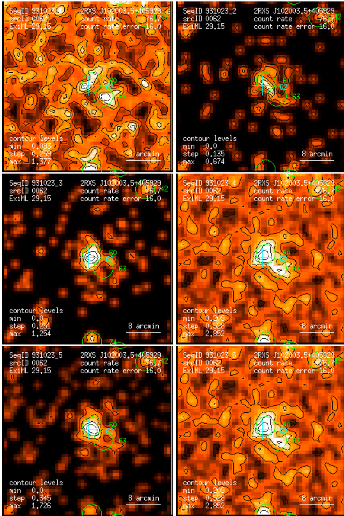
Figure 62: RASS 931023: detection 0062: band rate images, Gaussian filter: (1) PSPC channels 11 – 41, (2) 52 – 90, (3) 91 – 201, (4) 11 – 235, (5) 52 – 201, (6) 11 – 201. Broad band rates in counts/ks. Band rate contour levels in counts/ks/arcmin 2 .
