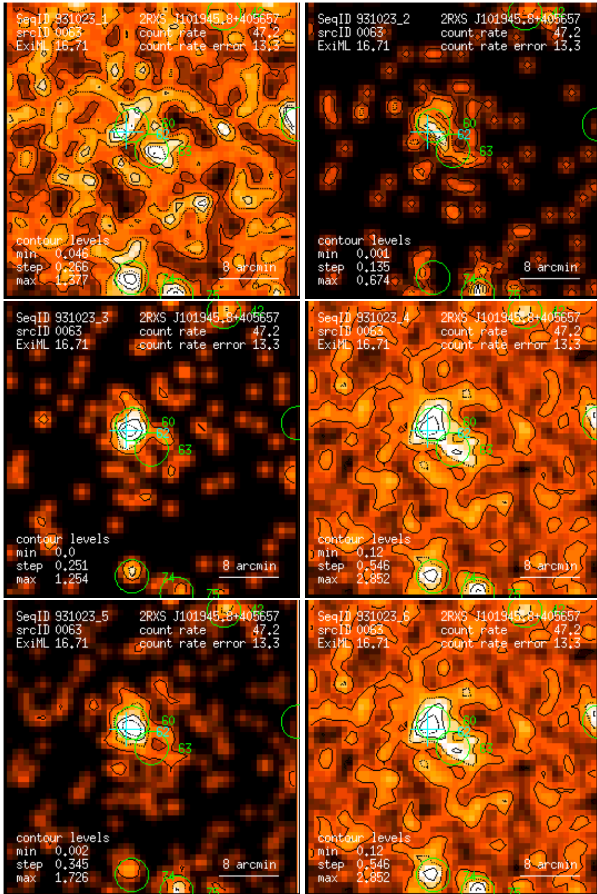
Figure 63: RASS 931023: detection 0063: band rate images, Gaussian filter: (1) PSPC channels 11 – 41, (2) 52 – 90, (3) 91 – 201, (4) 11 – 235, (5) 52 – 201, (6) 11 – 201. Broad band rates in counts/ks. Band rate contour levels in counts/ks/arcmin 2 .
