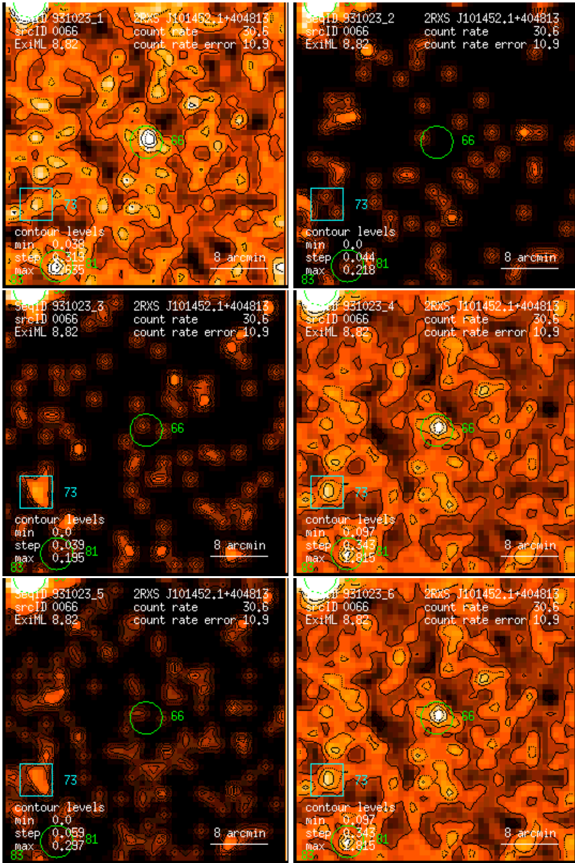
Figure 66: RASS 931023: detection 0066: band rate images, Gaussian filter: (1) PSPC channels 11 – 41, (2) 52 – 90, (3) 91 – 201, (4) 11 – 235, (5) 52 – 201, (6) 11 – 201. Broad band rates in counts/ks. Band rate contour levels in counts/ks/arcmin 2 .
