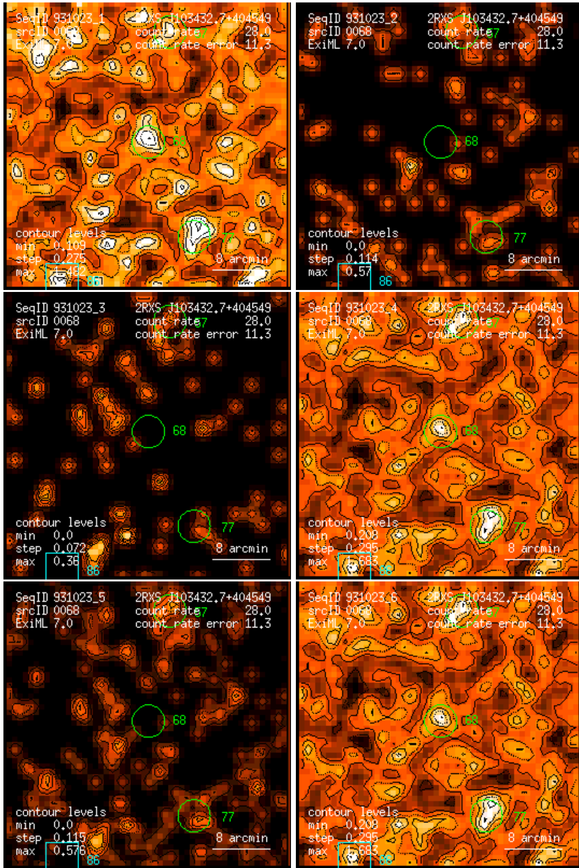
Figure 68: RASS 931023: detection 0068: band rate images, Gaussian filter: (1) PSPC channels 11 – 41, (2) 52 – 90, (3) 91 – 201, (4) 11 – 235, (5) 52 – 201, (6) 11 – 201. Broad band rates in counts/ks. Band rate contour levels in counts/ks/arcmin 2 .
