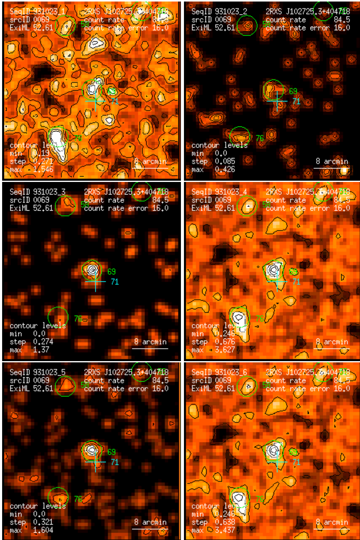
Figure 69: RASS 931023: detection 0069: band rate images, Gaussian filter: (1) PSPC channels 11 – 41, (2) 52 – 90, (3) 91 – 201, (4) 11 – 235, (5) 52 – 201, (6) 11 – 201. Broad band rates in counts/ks. Band rate contour levels in counts/ks/arcmin 2 .
