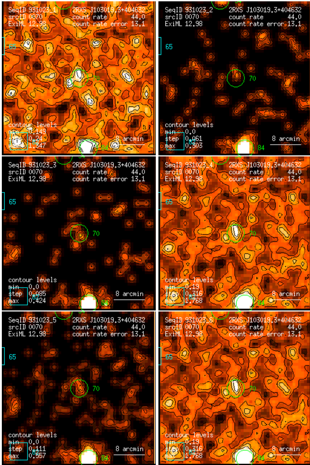
Figure 70: RASS 931023: detection 0070: band rate images, Gaussian filter: (1) PSPC channels 11 – 41, (2) 52 – 90, (3) 91 – 201, (4) 11 – 235, (5) 52 – 201, (6) 11 – 201. Broad band rates in counts/ks. Band rate contour levels in counts/ks/arcmin 2 .
