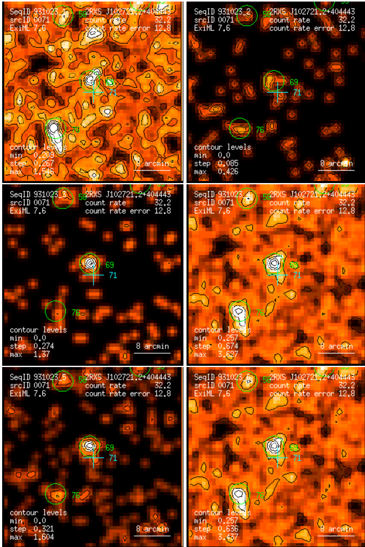
Figure 71: RASS 931023: detection 0071: band rate images, Gaussian filter: (1) PSPC channels 11 – 41, (2) 52 – 90, (3) 91 – 201, (4) 11 – 235, (5) 52 – 201, (6) 11 – 201. Broad band rates in counts/ks. Band rate contour levels in counts/ks/arcmin 2 .
