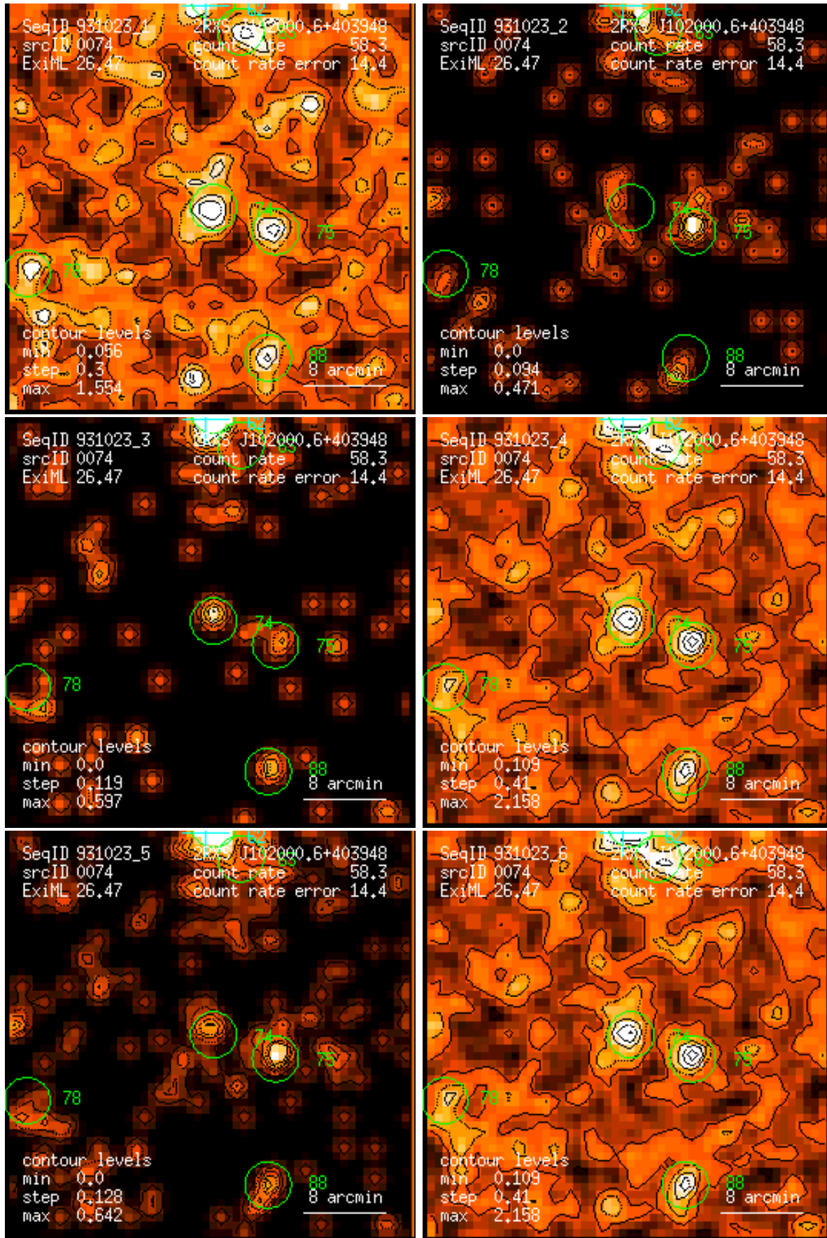
Figure 74: RASS 931023: detection 0074: band rate images, Gaussian filter: (1) PSPC channels 11 – 41, (2) 52 – 90, (3) 91 – 201, (4) 11 – 235, (5) 52 – 201, (6) 11 – 201. Broad band rates in counts/ks. Band rate contour levels in counts/ks/arcmin 2 .
