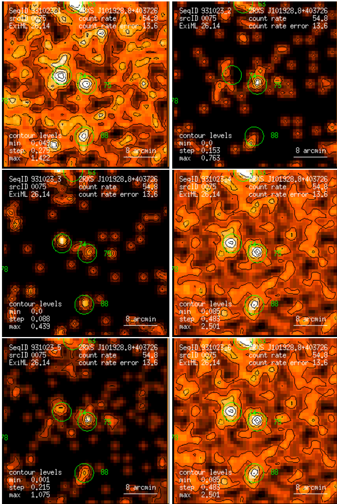
Figure 75: RASS 931023: detection 0075: band rate images, Gaussian filter: (1) PSPC channels 11 – 41, (2) 52 – 90, (3) 91 – 201, (4) 11 – 235, (5) 52 – 201, (6) 11 – 201. Broad band rates in counts/ks. Band rate contour levels in counts/ks/arcmin 2 .
