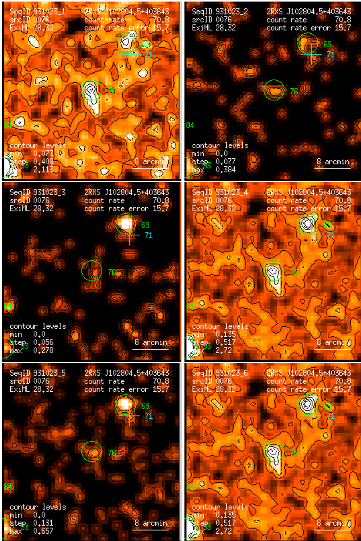
Figure 76: RASS 931023: detection 0076: band rate images, Gaussian filter: (1) PSPC channels 11 – 41, (2) 52 – 90, (3) 91 – 201, (4) 11 – 235, (5) 52 – 201, (6) 11 – 201. Broad band rates in counts/ks. Band rate contour levels in counts/ks/arcmin 2 .
