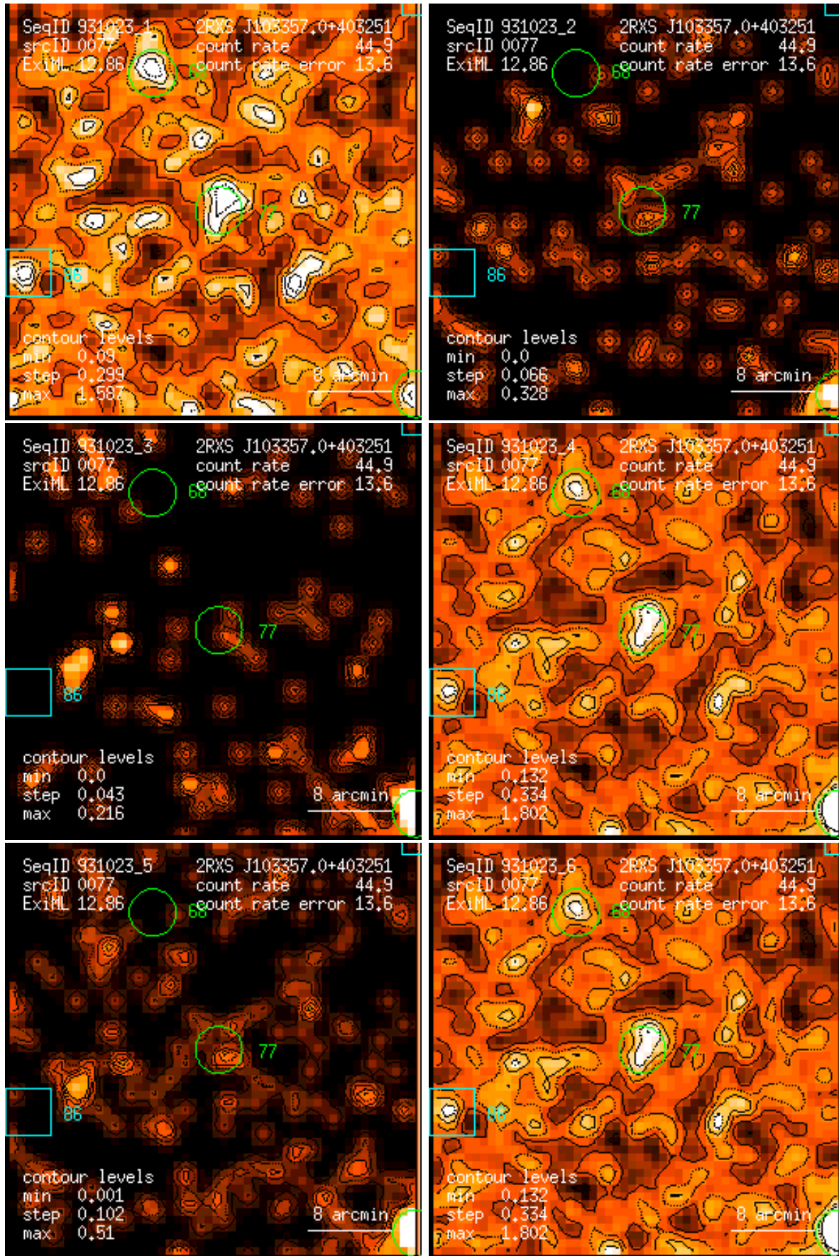
Figure 77: RASS 931023: detection 0077: band rate images, Gaussian filter: (1) PSPC channels 11 – 41, (2) 52 – 90, (3) 91 – 201, (4) 11 – 235, (5) 52 – 201, (6) 11 – 201. Broad band rates in counts/ks. Band rate contour levels in counts/ks/arcmin 2 .
