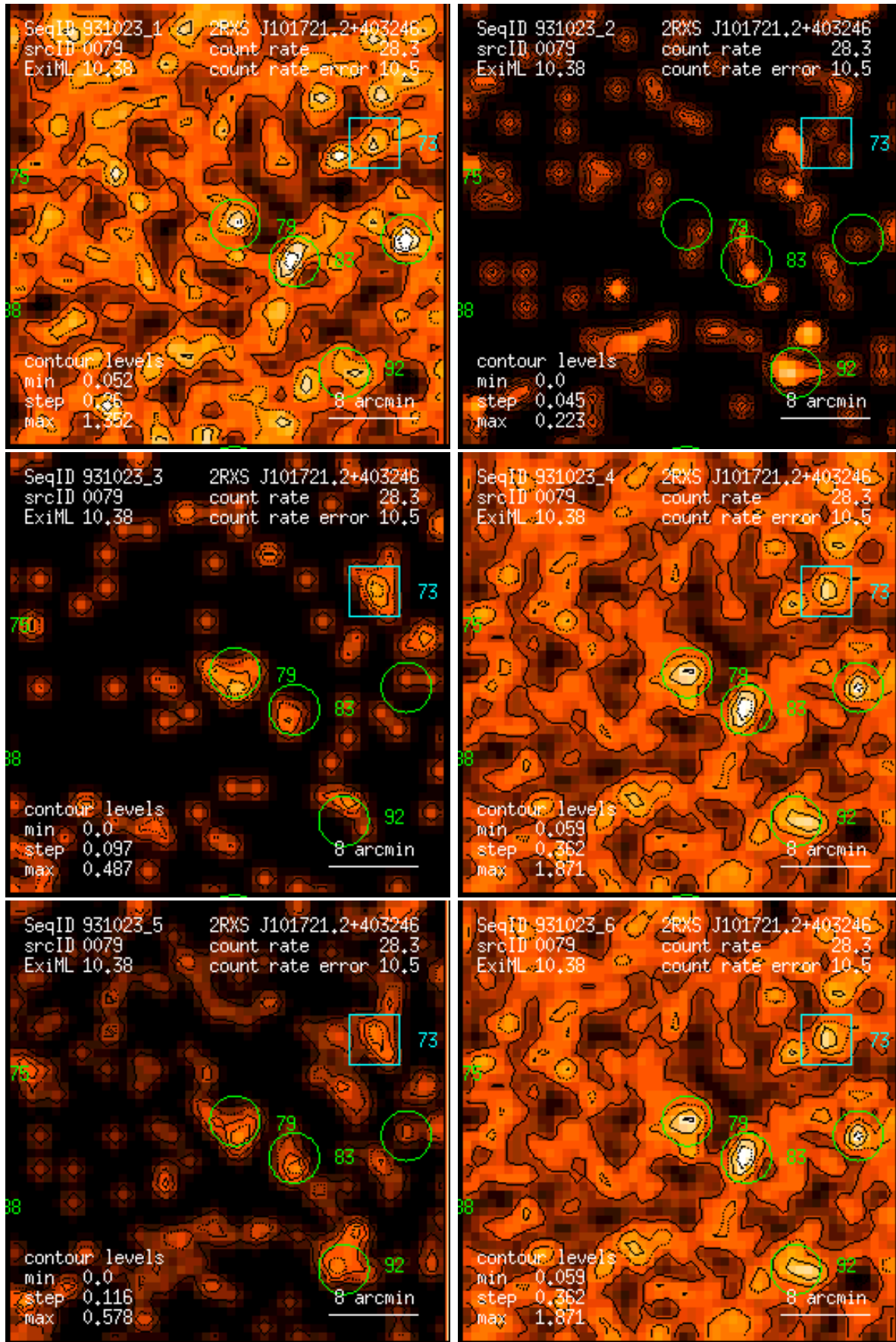
Figure 79: RASS 931023: detection 0079: band rate images, Gaussian filter: (1) PSPC channels 11 – 41, (2) 52 – 90, (3) 91 – 201, (4) 11 – 235, (5) 52 – 201, (6) 11 – 201. Broad band rates in counts/ks. Band rate contour levels in counts/ks/arcmin 2 .
