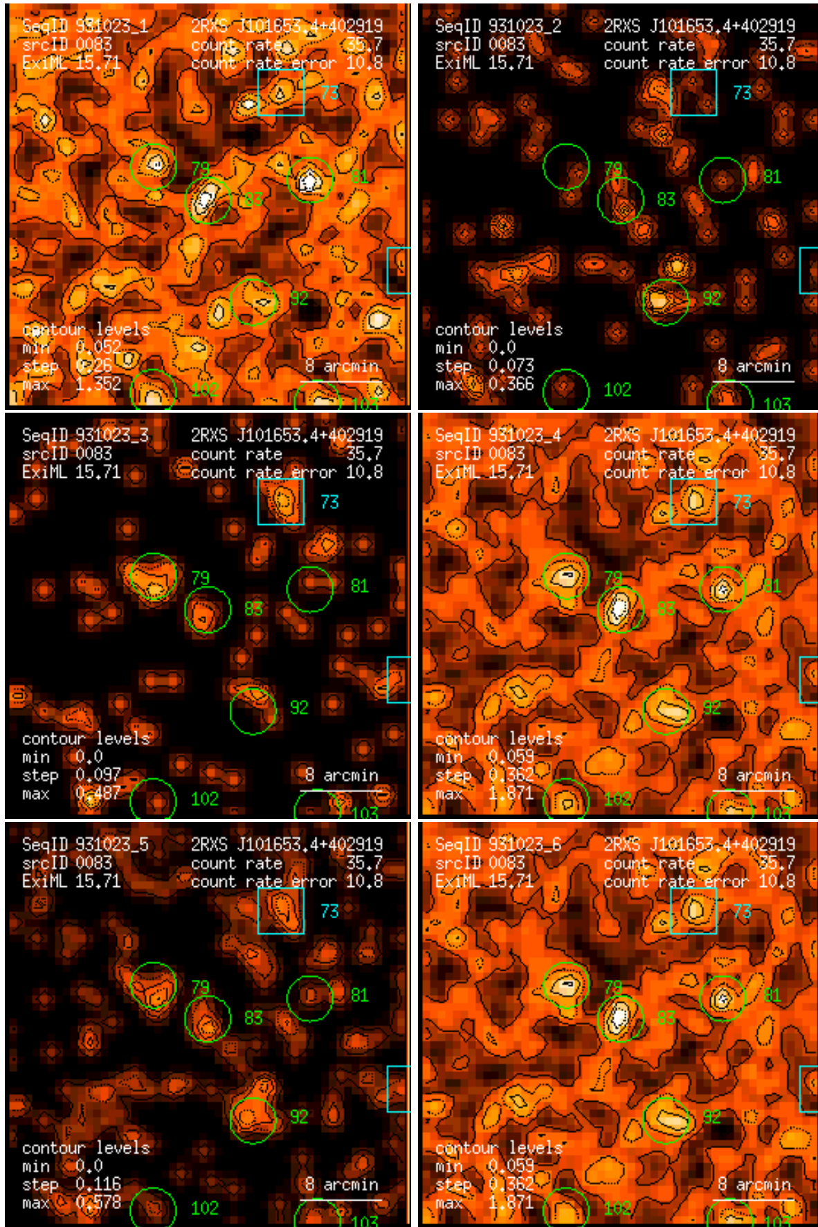
Figure 83: RASS 931023: detection 0083: band rate images, Gaussian filter: (1) PSPC channels 11 – 41, (2) 52 – 90, (3) 91 – 201, (4) 11 – 235, (5) 52 – 201, (6) 11 – 201. Broad band rates in counts/ks. Band rate contour levels in counts/ks/arcmin 2 .
