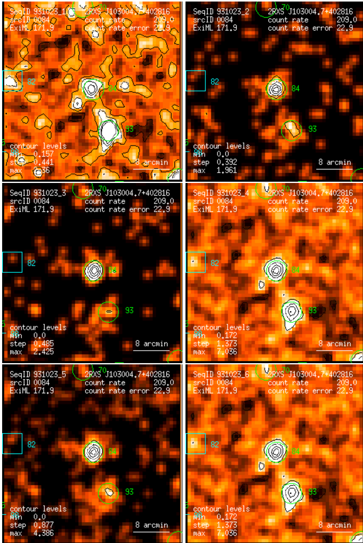
Figure 84: RASS 931023: detection 0084: band rate images, Gaussian filter: (1) PSPC channels 11 – 41, (2) 52 – 90, (3) 91 – 201, (4) 11 – 235, (5) 52 – 201, (6) 11 – 201. Broad band rates in counts/ks. Band rate contour levels in counts/ks/arcmin 2 .
