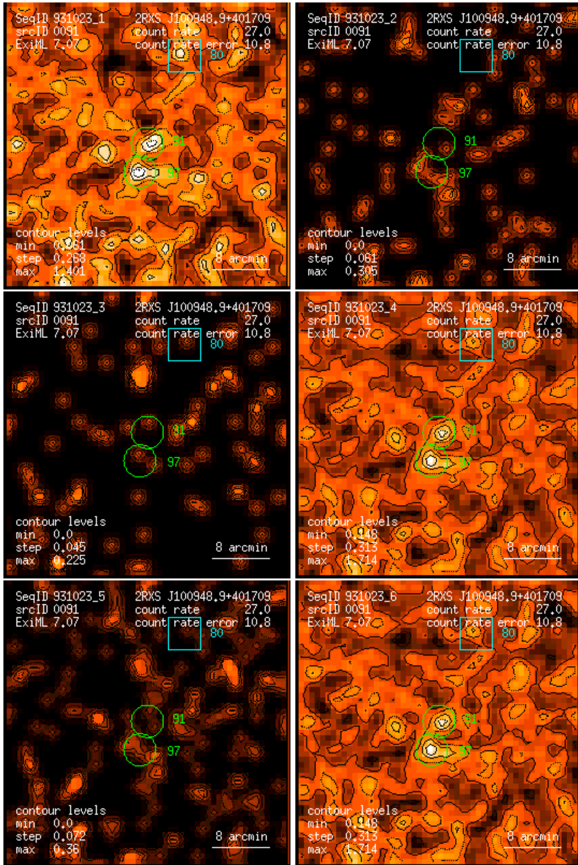
Figure 91: RASS 931023: detection 0091: band rate images, Gaussian filter: (1) PSPC channels 11 – 41, (2) 52 – 90, (3) 91 – 201, (4) 11 – 235, (5) 52 – 201, (6) 11 – 201. Broad band rates in counts/ks. Band rate contour levels in counts/ks/arcmin 2 .
