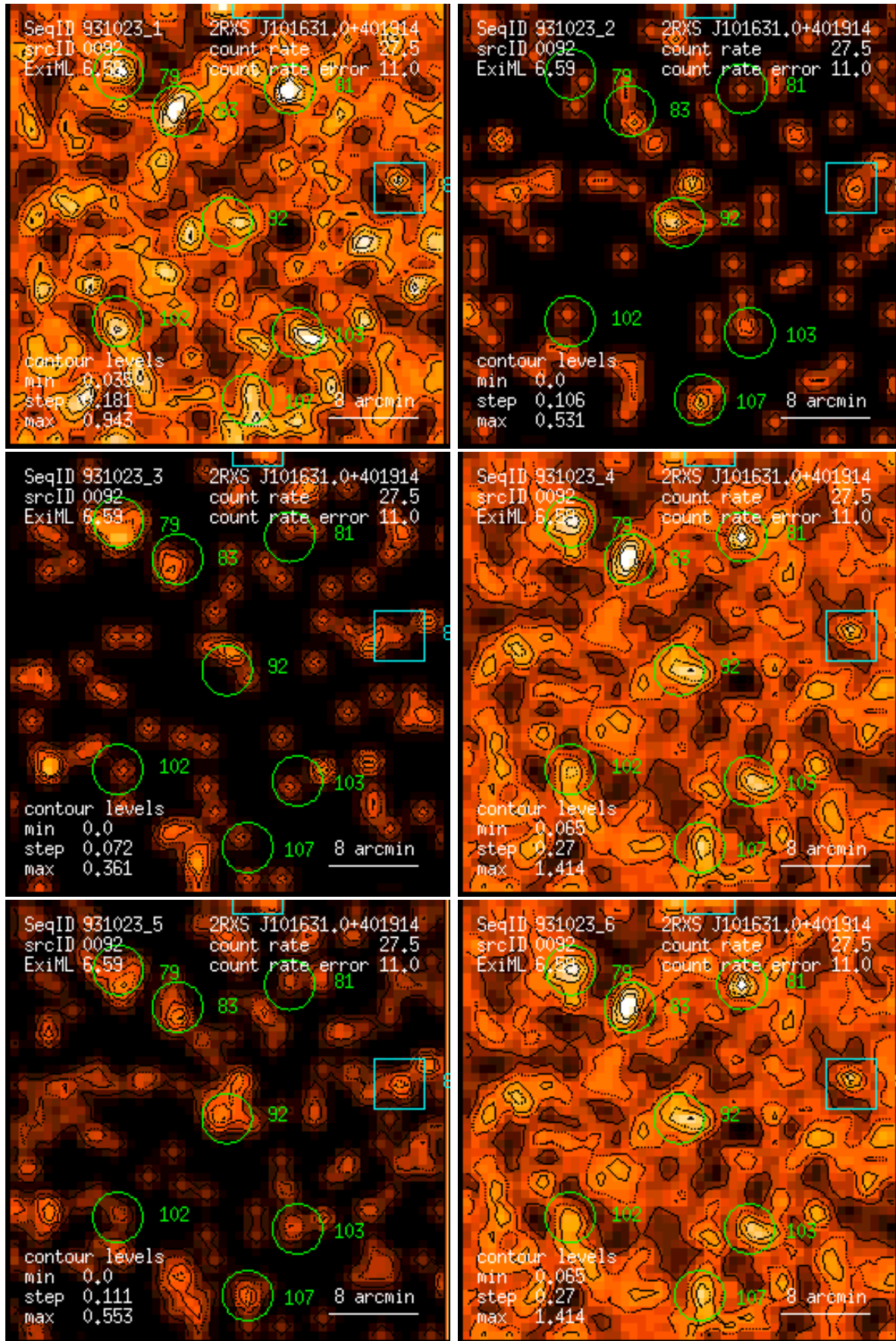
Figure 92: RASS 931023: detection 0092: band rate images, Gaussian filter: (1) PSPC channels 11 – 41, (2) 52 – 90, (3) 91 – 201, (4) 11 – 235, (5) 52 – 201, (6) 11 – 201. Broad band rates in counts/ks. Band rate contour levels in counts/ks/arcmin 2 .
