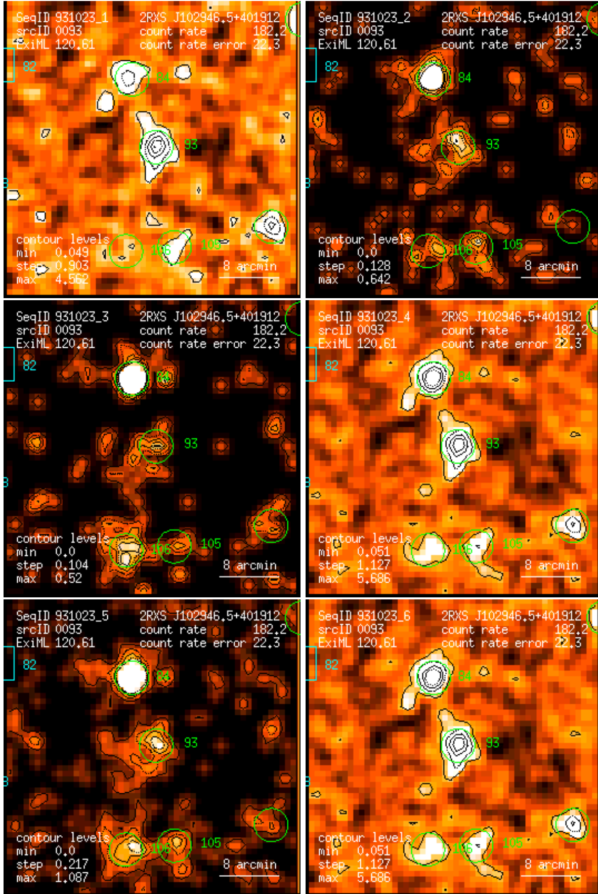
Figure 93: RASS 931023: detection 0093: band rate images, Gaussian filter: (1) PSPC channels 11 – 41, (2) 52 – 90, (3) 91 – 201, (4) 11 – 235, (5) 52 – 201, (6) 11 – 201. Broad band rates in counts/ks. Band rate contour levels in counts/ks/arcmin 2 .
