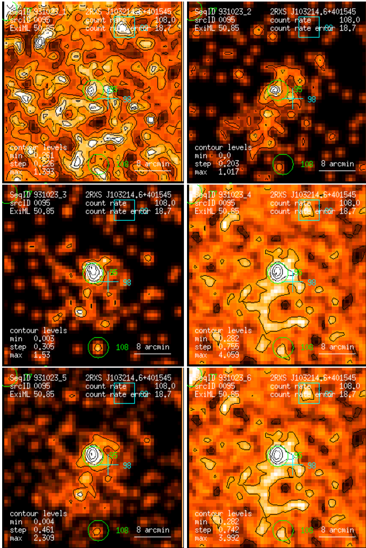
Figure 95: RASS 931023: detection 0095: band rate images, Gaussian filter: (1) PSPC channels 11 – 41, (2) 52 – 90, (3) 91 – 201, (4) 11 – 235, (5) 52 – 201, (6) 11 – 201. Broad band rates in counts/ks. Band rate contour levels in counts/ks/arcmin 2 .
