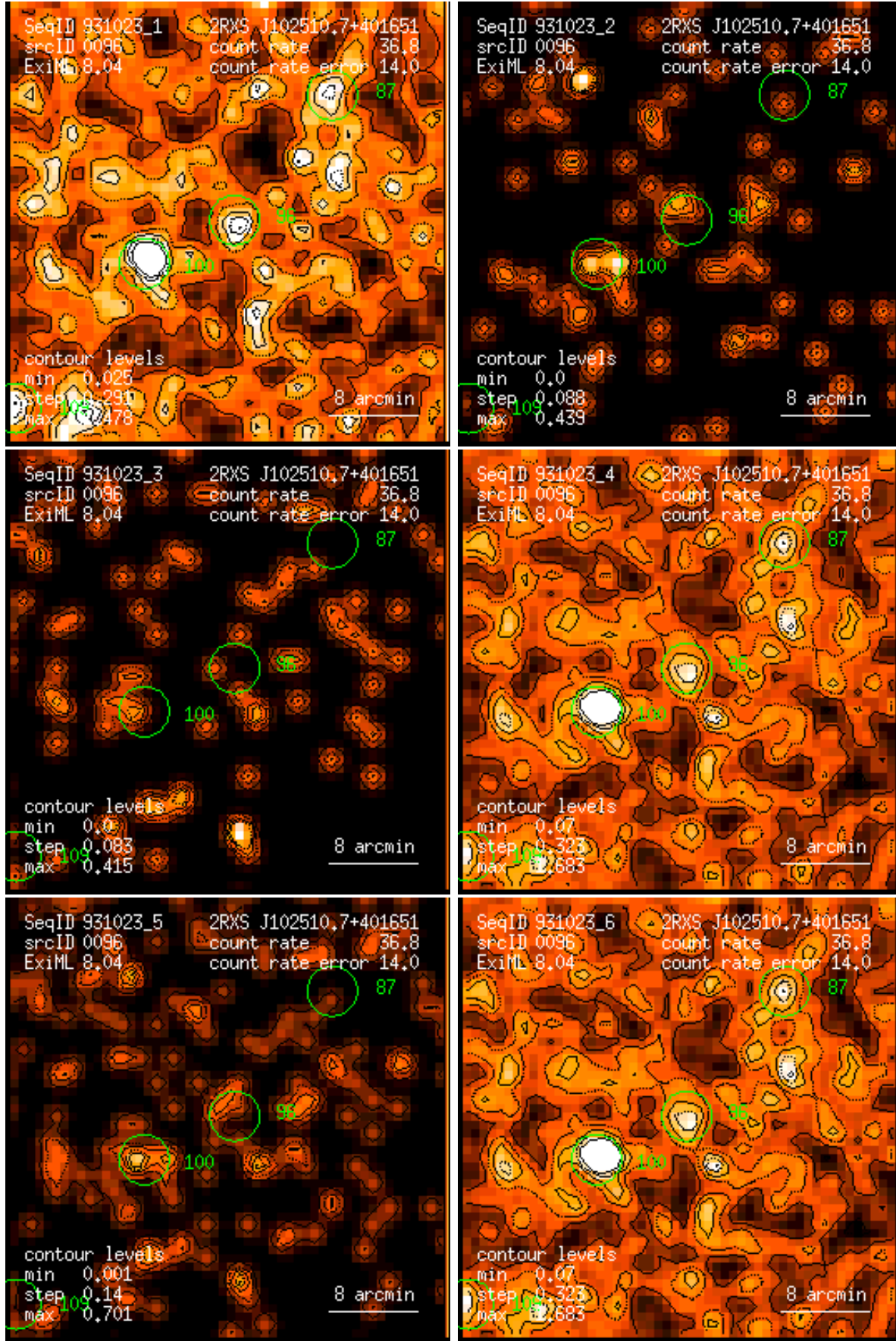
Figure 96: RASS 931023: detection 0096: band rate images, Gaussian filter: (1) PSPC channels 11 – 41, (2) 52 – 90, (3) 91 – 201, (4) 11 – 235, (5) 52 – 201, (6) 11 – 201. Broad band rates in counts/ks. Band rate contour levels in counts/ks/arcmin 2 .
