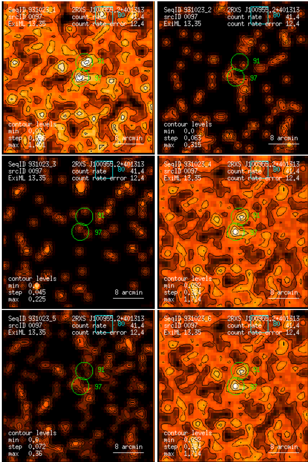
Figure 97: RASS 931023: detection 0097: band rate images, Gaussian filter: (1) PSPC channels 11 – 41, (2) 52 – 90, (3) 91 – 201, (4) 11 – 235, (5) 52 – 201, (6) 11 – 201. Broad band rates in counts/ks. Band rate contour levels in counts/ks/arcmin 2 .
