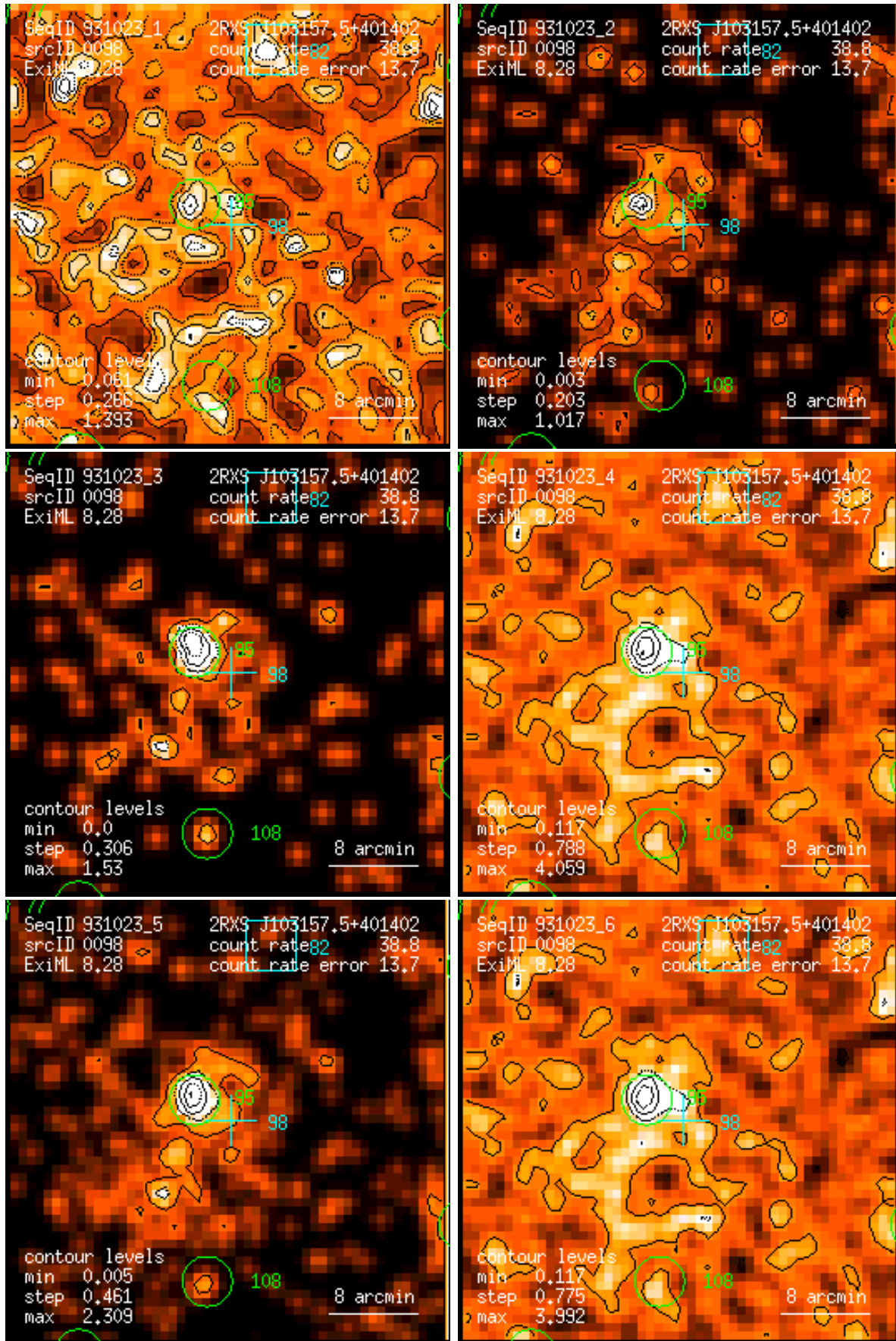
Figure 98: RASS 931023: detection 0098: band rate images, Gaussian filter: (1) PSPC channels 11 – 41, (2) 52 – 90, (3) 91 – 201, (4) 11 – 235, (5) 52 – 201, (6) 11 – 201. Broad band rates in counts/ks. Band rate contour levels in counts/ks/arcmin 2 .
