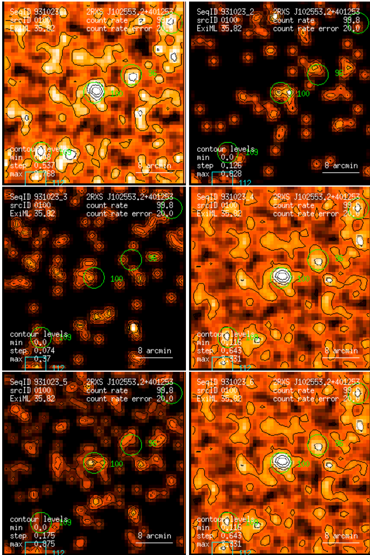
Figure 100: RASS 931023: detection 0100: band rate images, Gaussian filter: (1) PSPC channels 11 – 41, (2) 52 – 90, (3) 91 – 201, (4) 11 – 235, (5) 52 – 201, (6) 11 – 201. Broad band rates in counts/ks. Band rate contour levels in counts/ks/arcmin 2 .
