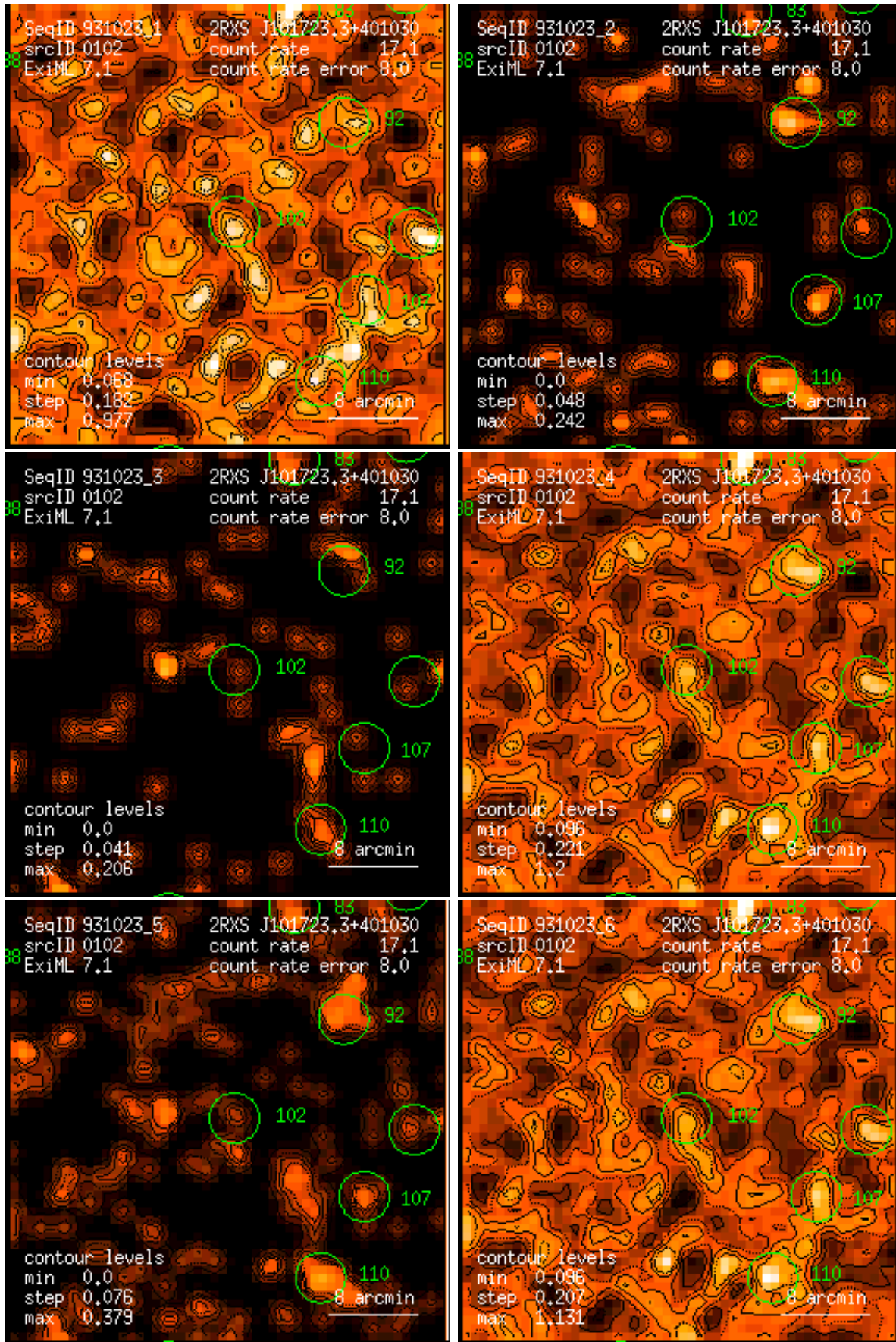
Figure 102: RASS 931023: detection 0102: band rate images, Gaussian filter: (1) PSPC channels 11 – 41, (2) 52 – 90, (3) 91 – 201, (4) 11 – 235, (5) 52 – 201, (6) 11 – 201. Broad band rates in counts/ks. Band rate contour levels in counts/ks/arcmin 2 .
