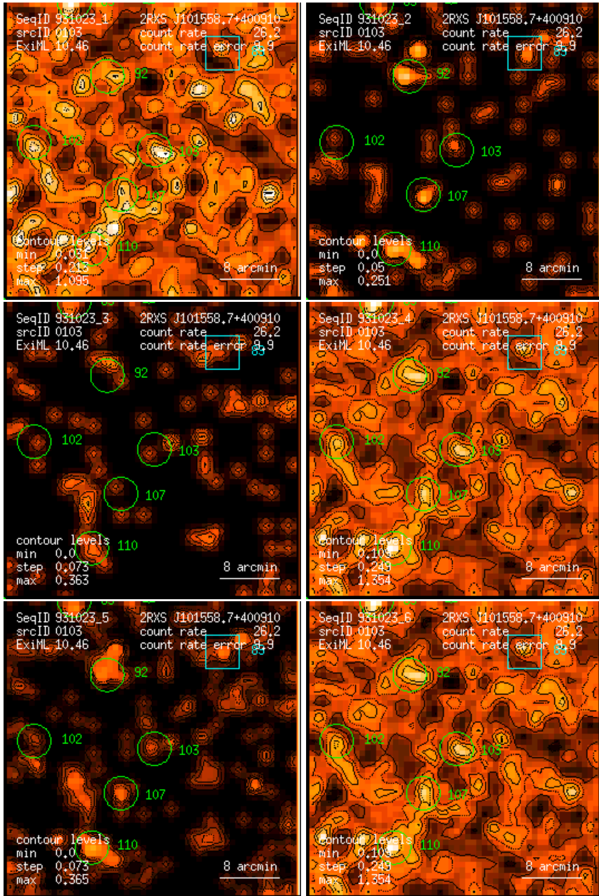
Figure 103: RASS 931023: detection 0103: band rate images, Gaussian filter: (1) PSPC channels 11 – 41, (2) 52 – 90, (3) 91 – 201, (4) 11 – 235, (5) 52 – 201, (6) 11 – 201. Broad band rates in counts/ks. Band rate contour levels in counts/ks/arcmin 2 .
