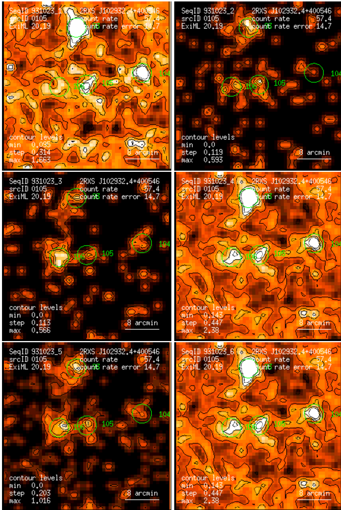
Figure 105: RASS 931023: detection 0105: band rate images, Gaussian filter: (1) PSPC channels 11 – 41, (2) 52 – 90, (3) 91 – 201, (4) 11 – 235, (5) 52 – 201, (6) 11 – 201. Broad band rates in counts/ks. Band rate contour levels in counts/ks/arcmin 2 .
