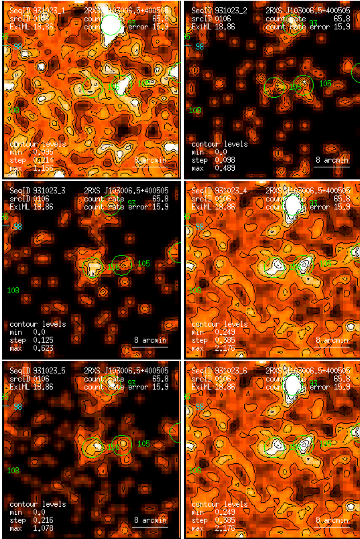
Figure 106: RASS 931023: detection 0106: band rate images, Gaussian filter: (1) PSPC channels 11 – 41, (2) 52 – 90, (3) 91 – 201, (4) 11 – 235, (5) 52 – 201, (6) 11 – 201. Broad band rates in counts/ks. Band rate contour levels in counts/ks/arcmin 2 .
