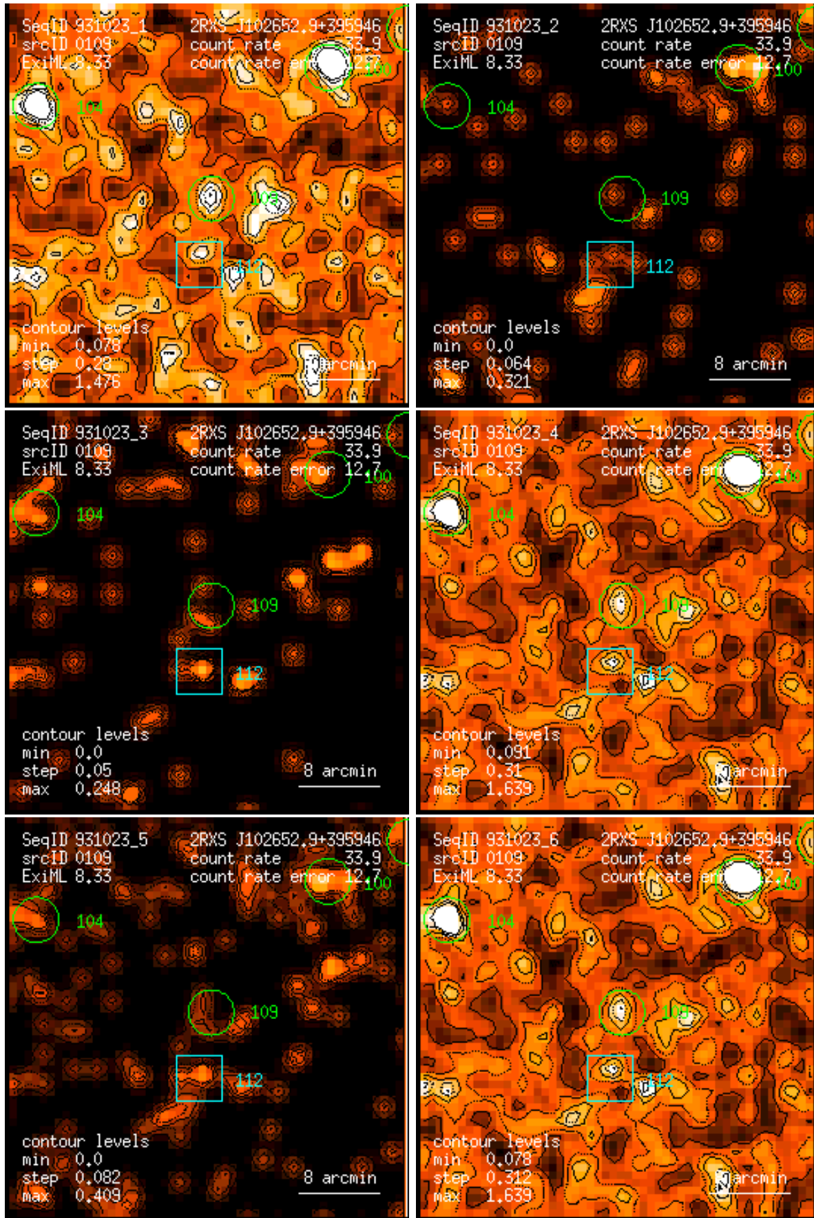
Figure 109: RASS 931023: detection 0109: band rate images, Gaussian filter: (1) PSPC channels 11 – 41, (2) 52 – 90, (3) 91 – 201, (4) 11 – 235, (5) 52 – 201, (6) 11 – 201. Broad band rates in counts/ks. Band rate contour levels in counts/ks/arcmin 2 .
