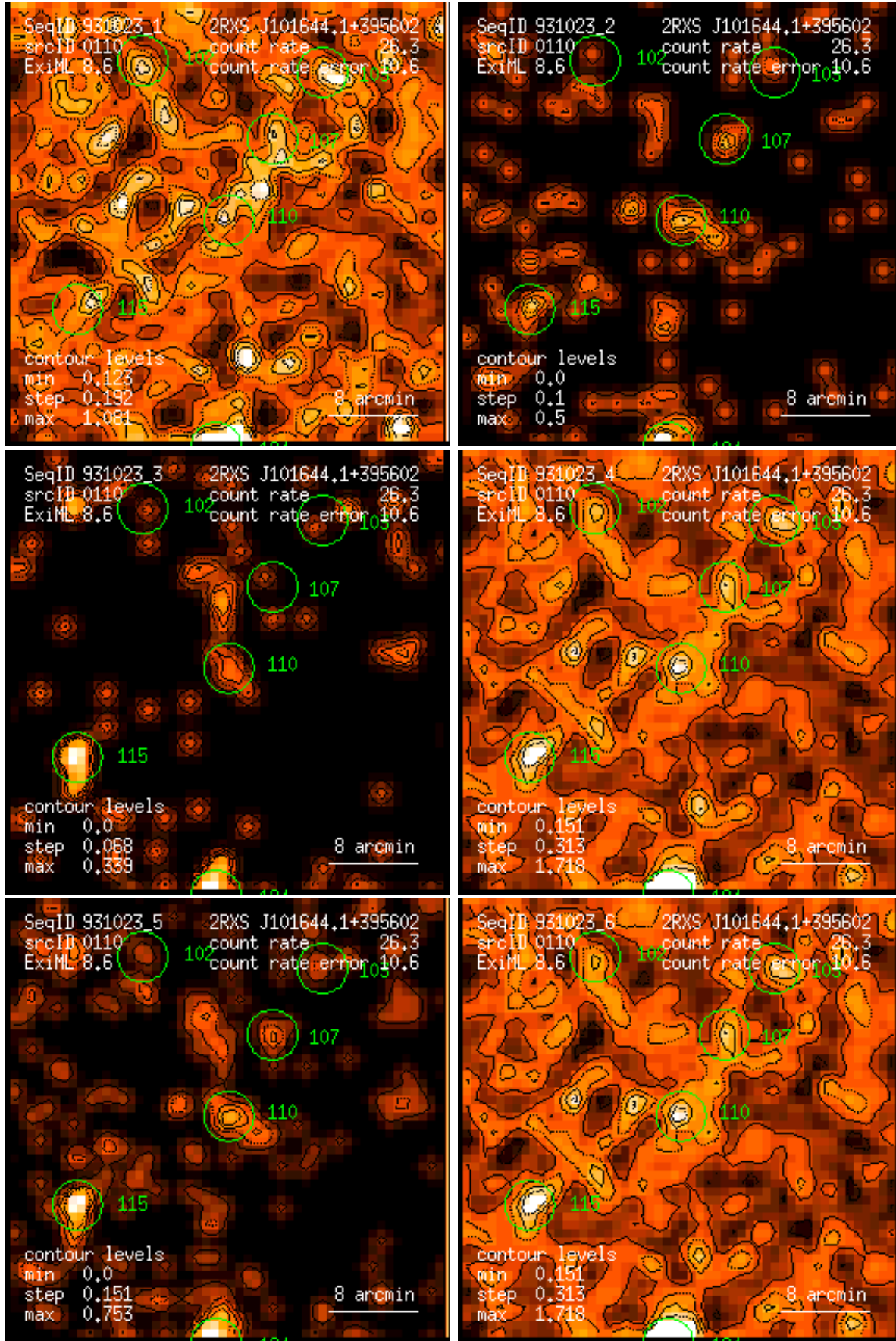
Figure 110: RASS 931023: detection 0110: band rate images, Gaussian filter: (1) PSPC channels 11 – 41, (2) 52 – 90, (3) 91 – 201, (4) 11 – 235, (5) 52 – 201, (6) 11 – 201. Broad band rates in counts/ks. Band rate contour levels in counts/ks/arcmin 2 .
