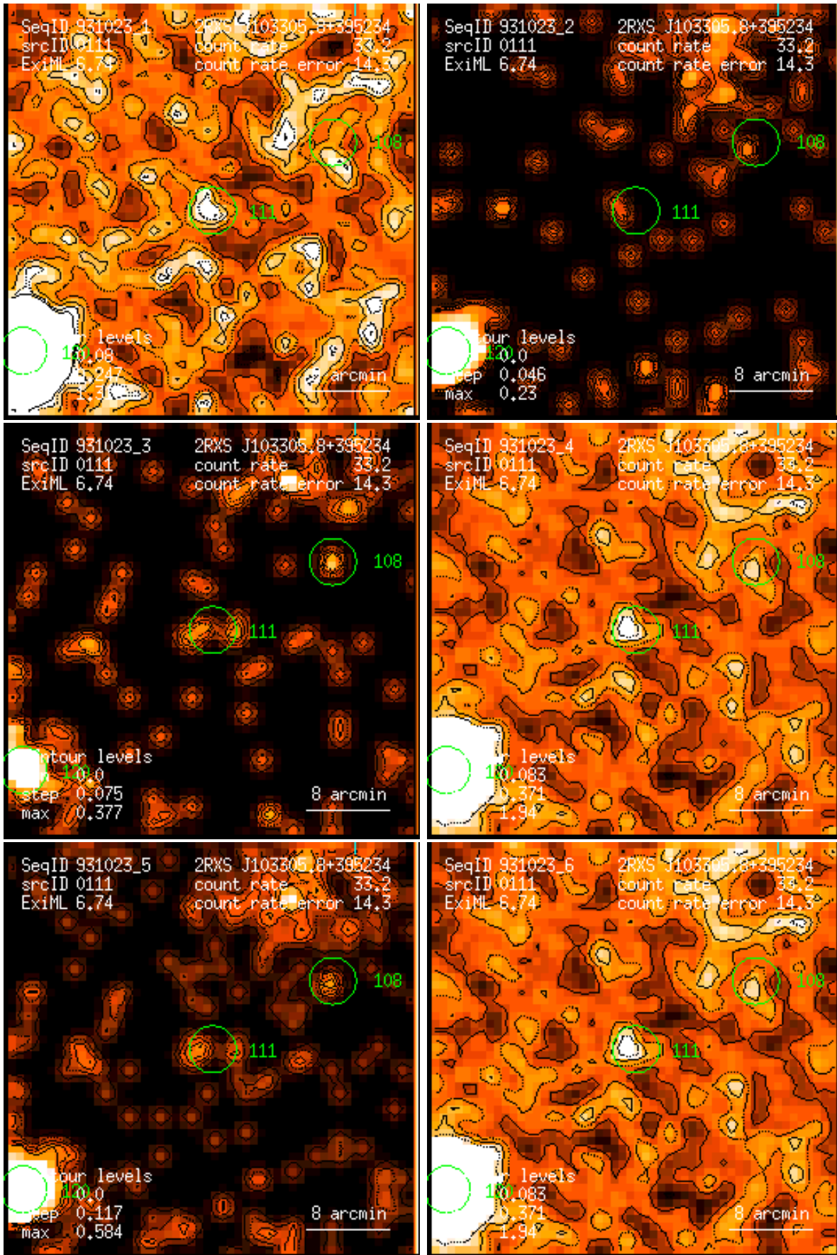
Figure 111: RASS 931023: detection 0111: band rate images, Gaussian filter: (1) PSPC channels 11 – 41, (2) 52 – 90, (3) 91 – 201, (4) 11 – 235, (5) 52 – 201, (6) 11 – 201. Broad band rates in counts/ks. Band rate contour levels in counts/ks/arcmin 2 .
