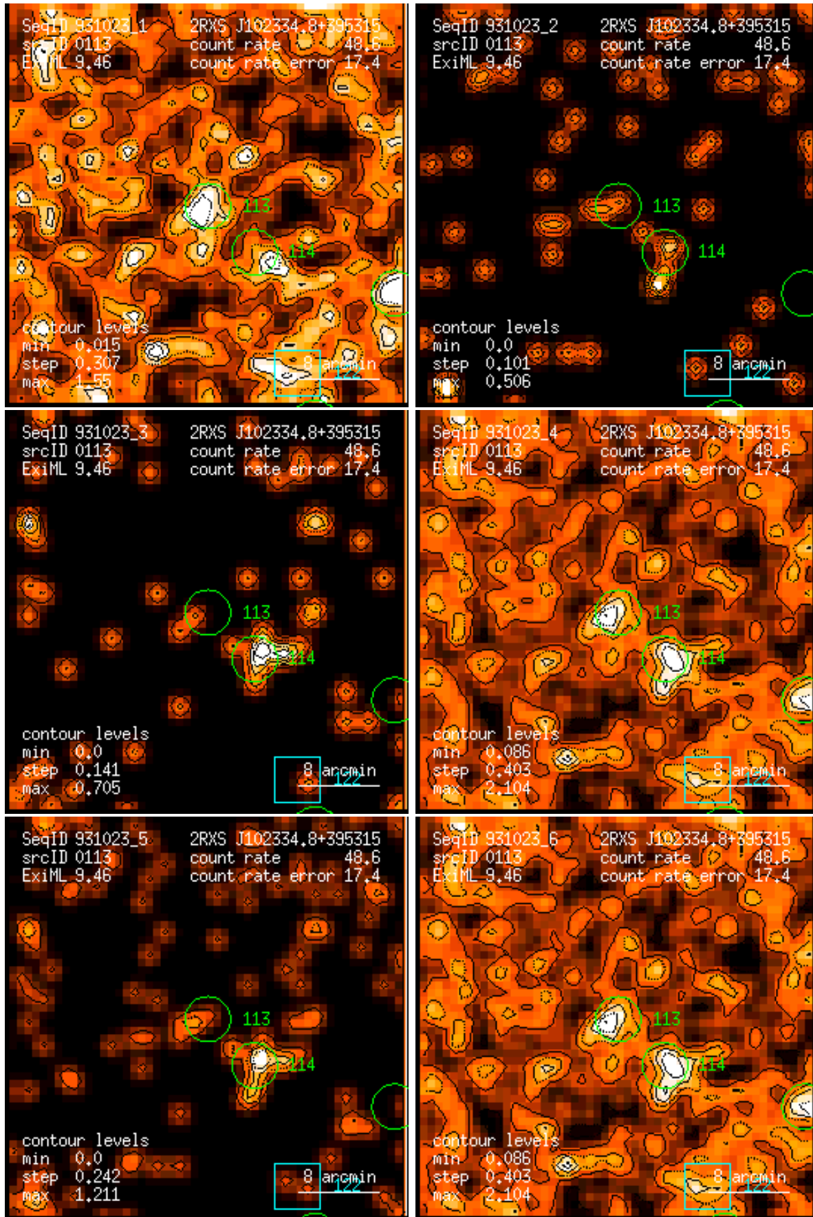
Figure 113: RASS 931023: detection 0113: band rate images, Gaussian filter: (1) PSPC channels 11 – 41, (2) 52 – 90, (3) 91 – 201, (4) 11 – 235, (5) 52 – 201, (6) 11 – 201. Broad band rates in counts/ks. Band rate contour levels in counts/ks/arcmin 2 .
