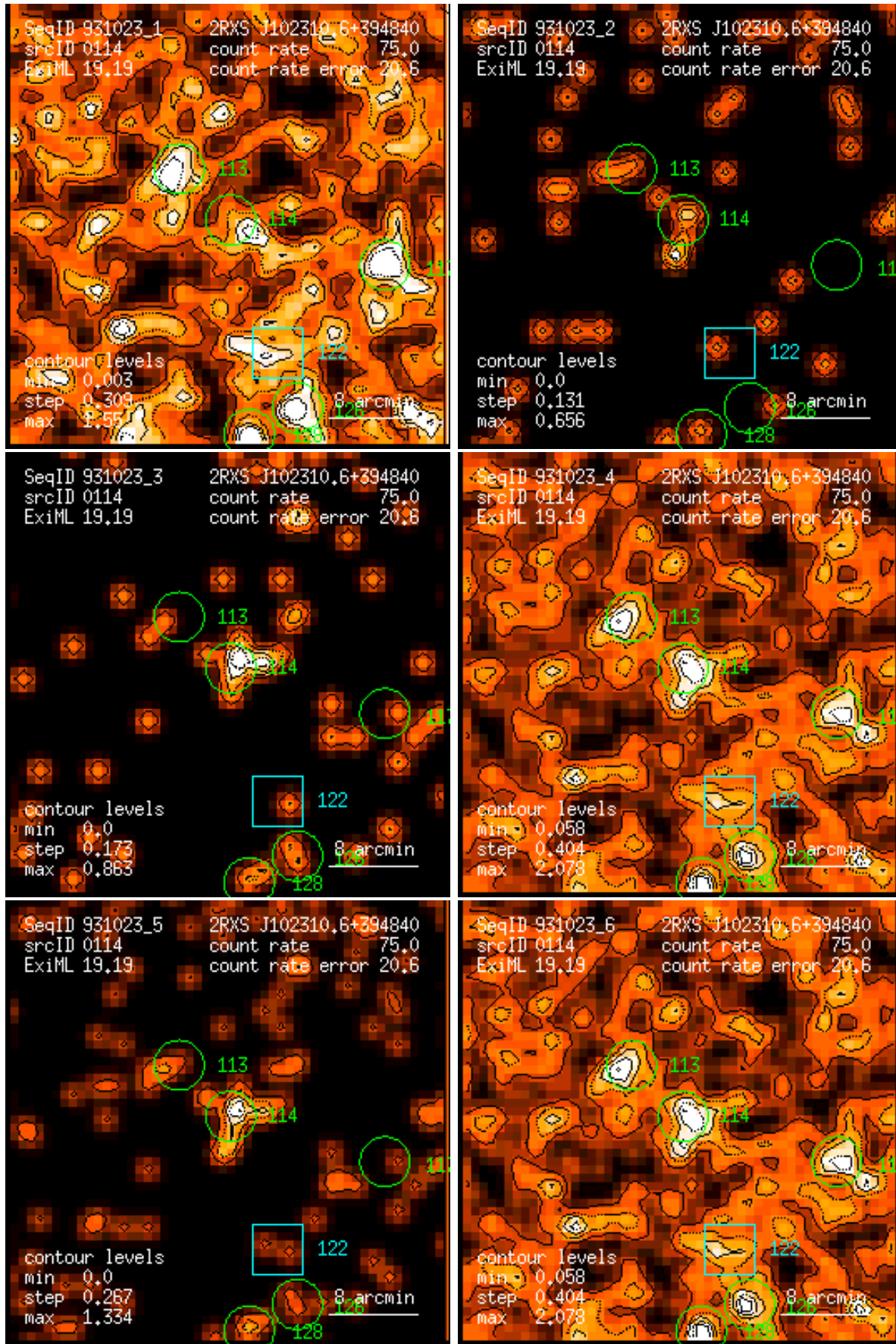
Figure 114: RASS 931023: detection 0114: band rate images, Gaussian filter: (1) PSPC channels 11 – 41, (2) 52 – 90, (3) 91 – 201, (4) 11 – 235, (5) 52 – 201, (6) 11 – 201. Broad band rates in counts/ks. Band rate contour levels in counts/ks/arcmin 2 .
