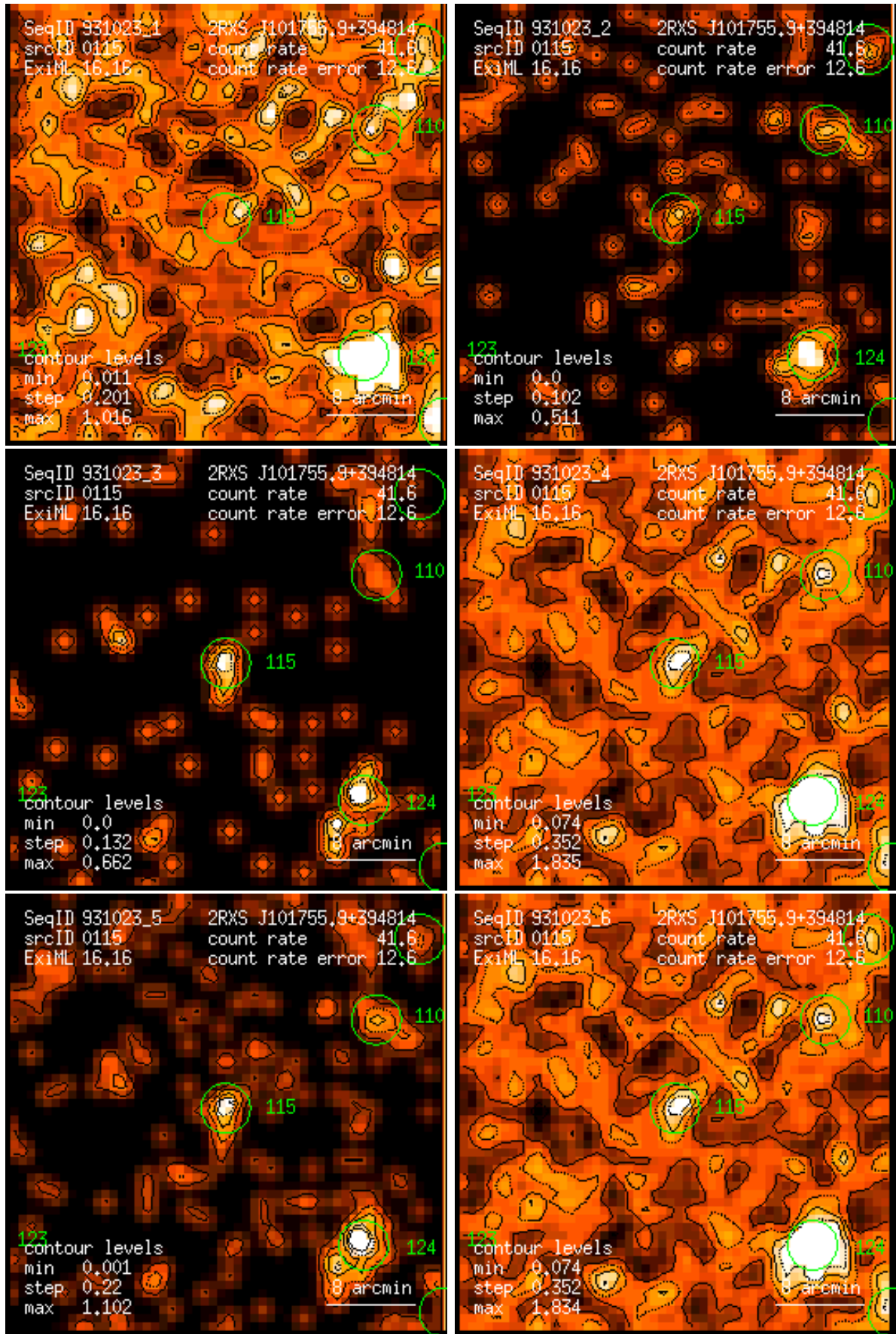
Figure 115: RASS 931023: detection 0115: band rate images, Gaussian filter: (1) PSPC channels 11 – 41, (2) 52 – 90, (3) 91 – 201, (4) 11 – 235, (5) 52 – 201, (6) 11 – 201. Broad band rates in counts/ks. Band rate contour levels in counts/ks/arcmin 2 .
