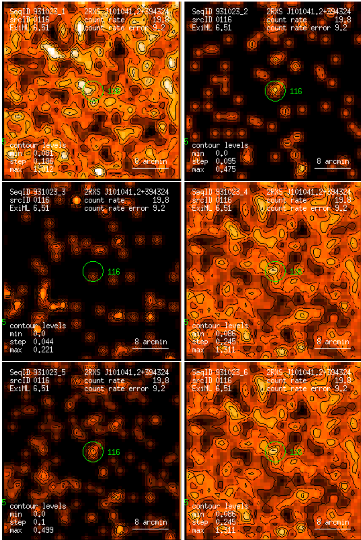
Figure 116: RASS 931023: detection 0116: band rate images, Gaussian filter: (1) PSPC channels 11 – 41, (2) 52 – 90, (3) 91 – 201, (4) 11 – 235, (5) 52 – 201, (6) 11 – 201. Broad band rates in counts/ks. Band rate contour levels in counts/ks/arcmin 2 .
