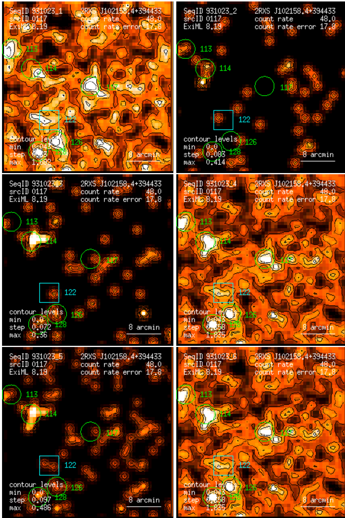
Figure 117: RASS 931023: detection 0117: band rate images, Gaussian filter: (1) PSPC channels 11 – 41, (2) 52 – 90, (3) 91 – 201, (4) 11 – 235, (5) 52 – 201, (6) 11 – 201. Broad band rates in counts/ks. Band rate contour levels in counts/ks/arcmin 2 .
