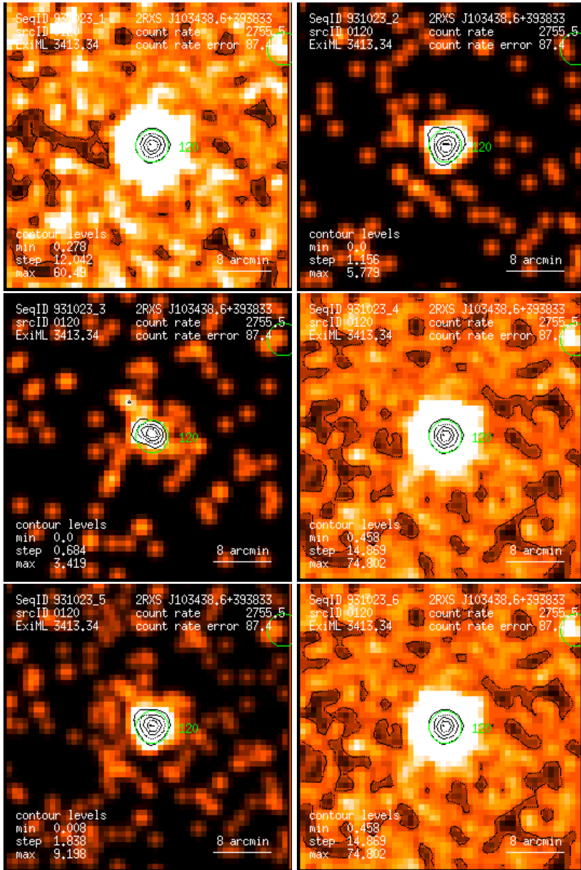
Figure 120: RASS 931023: detection 0120: band rate images, Gaussian filter: (1) PSPC channels 11 – 41, (2) 52 – 90, (3) 91 – 201, (4) 11 – 235, (5) 52 – 201, (6) 11 – 201. Broad band rates in counts/ks. Band rate contour levels in counts/ks/arcmin 2 .
