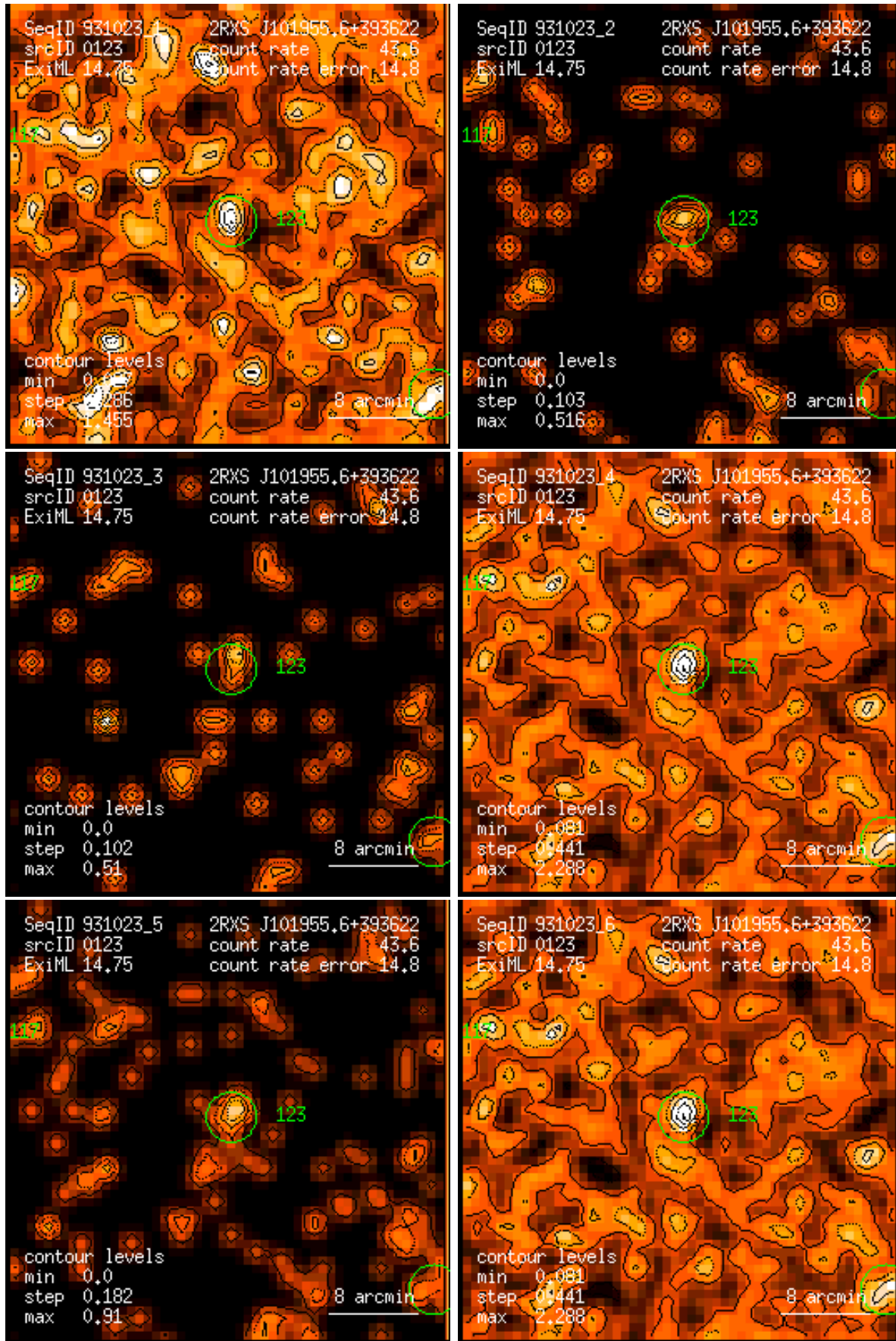
Figure 123: RASS 931023: detection 0123: band rate images, Gaussian filter: (1) PSPC channels 11 – 41, (2) 52 – 90, (3) 91 – 201, (4) 11 – 235, (5) 52 – 201, (6) 11 – 201. Broad band rates in counts/ks. Band rate contour levels in counts/ks/arcmin 2 .
