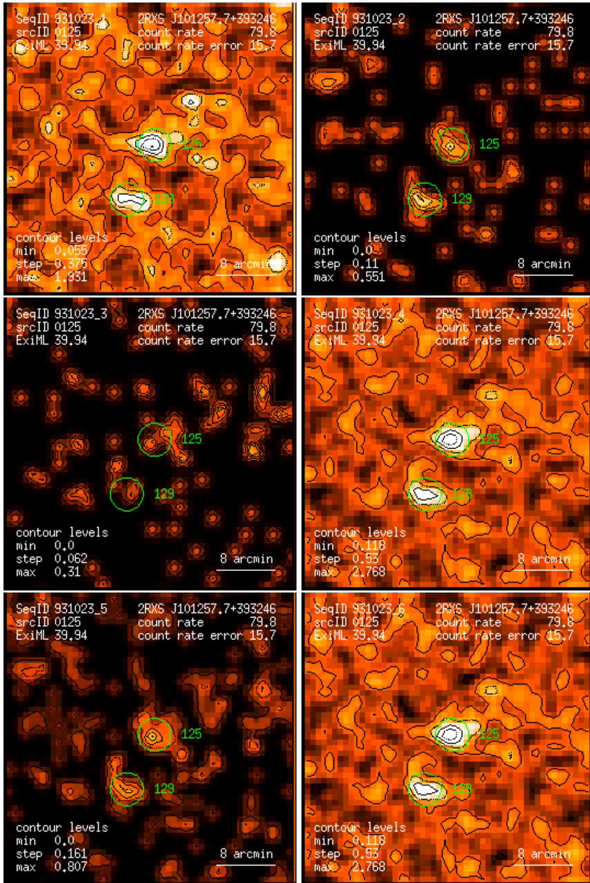
Figure 125: RASS 931023: detection 0125: band rate images, Gaussian filter: (1) PSPC channels 11 – 41, (2) 52 – 90, (3) 91 – 201, (4) 11 – 235, (5) 52 – 201, (6) 11 – 201. Broad band rates in counts/ks. Band rate contour levels in counts/ks/arcmin 2 .
