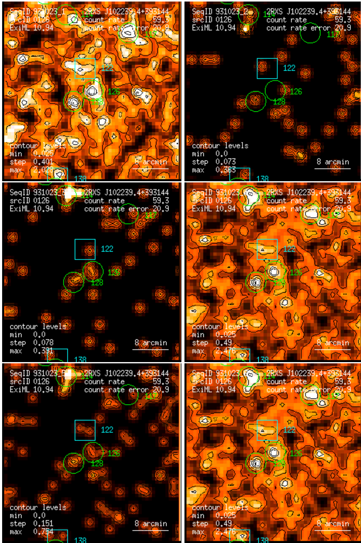
Figure 126: RASS 931023: detection 0126: band rate images, Gaussian filter: (1) PSPC channels 11 – 41, (2) 52 – 90, (3) 91 – 201, (4) 11 – 235, (5) 52 – 201, (6) 11 – 201. Broad band rates in counts/ks. Band rate contour levels in counts/ks/arcmin 2 .
